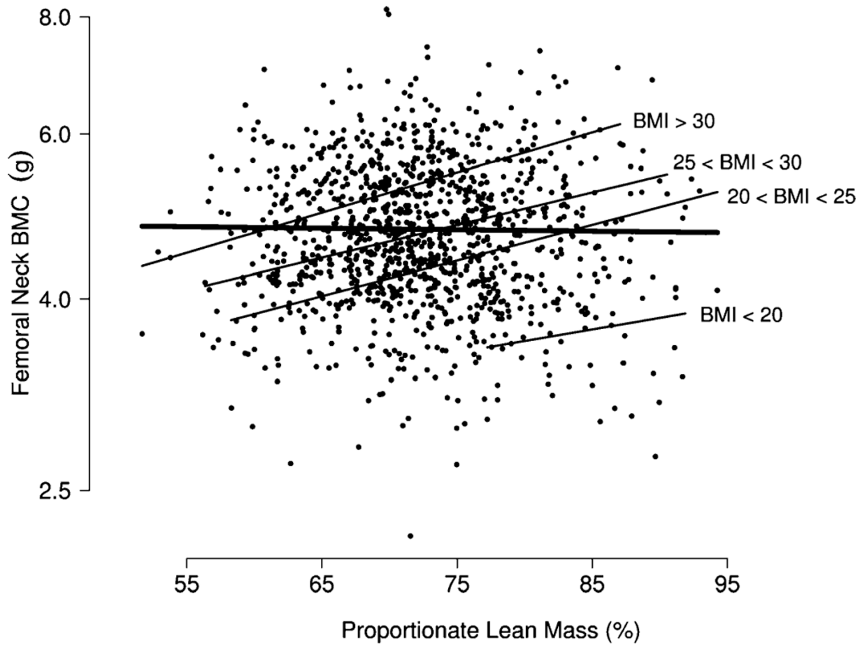
Fig. 3. Femoral neck BMC versus proportionate lean mass. There is little marginal association (thick line). However, when subjects are grouped according to BMI ( \text{kg}/\text{m}^2 ), the sharper association between lean mass and BMC becomes clear (thin lines)
