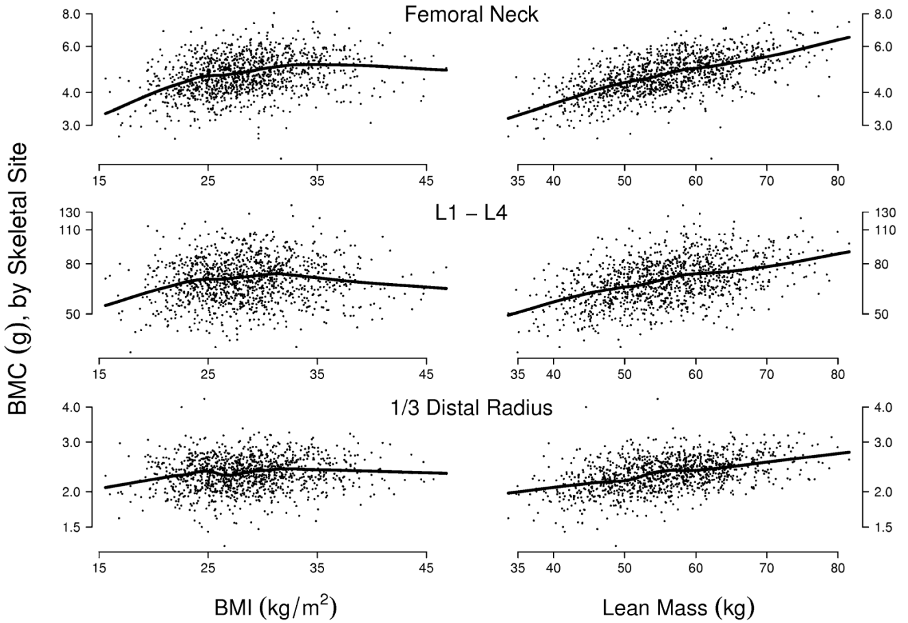
Fig. 1. Bone mineral content (BMC) versus body mass index (BMI) and lean mass, by skeletal site. Semiparametric scatter-plot smooths (black lines) indicate that BMI displays a positive association with BMC up to approximately 35 kg/m 2 , whereas the association between total lean mass and BMC is positive over the entire range of lean mass values. The association between BMC and body composition is weaker at the wrist than at other sites
