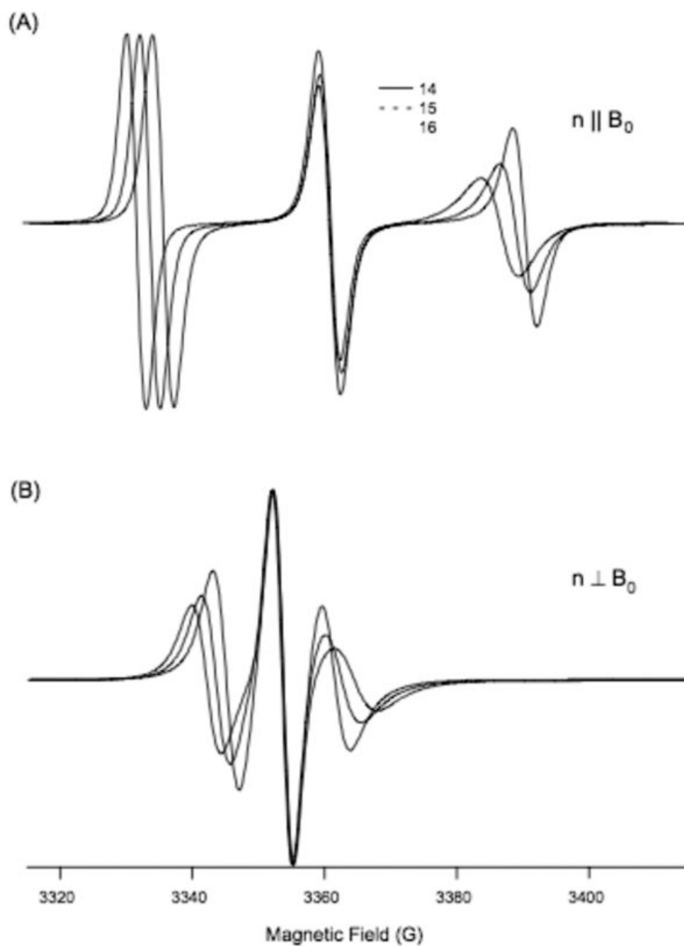
Figure 1. Simulation of EPR spectra for residues 14-16 demonstrating how the A_{\text{exp}} values change between these residues. (A) Parallel aligned (B) perpendicularly aligned with respect to the direction of magnetic field ( B_0 ).
