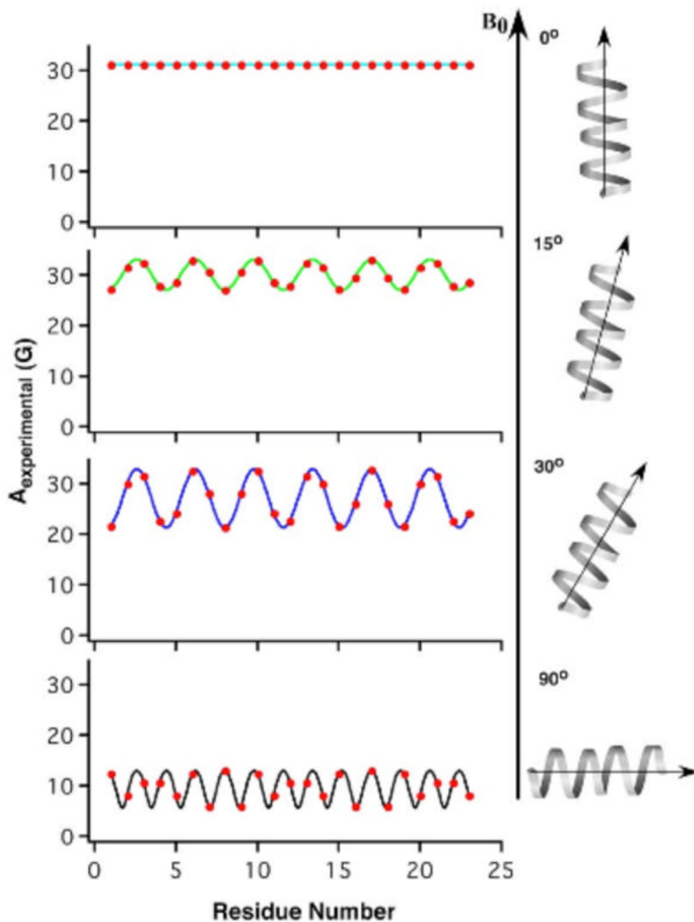
Figure 2. Hyperfine waves as a function of helical tilt angle, using predefined values for A_{\parallel} (33.3 G), A_{\perp} (5.6 G), \beta_D (21°), and \alpha_D at residue 18 (-10°).
