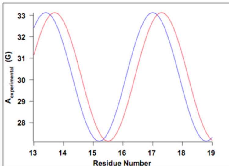
Figure 5. Hyperfine wave as a function of residue number and showing a shift in the hyperfine waves due to changing the \alpha_D frame. The blue wave represents the correct \alpha_D frame, while the red wave is out of phase by 30^\circ . When the wave is out of phase, it shifts either to the right or to the left and causes the corresponding helical tilt angle ranges to become incompatible with each other as a result, which can be seen in Table 3.
