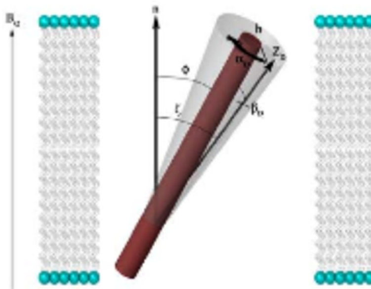
Figure 3. Illustration of an \alpha -helix with attached TOAC spin label and applied magnetic field. \phi represents the helical tilt angle, \zeta , (equal to \psi in the parallel orientation) is the director tilt angle, which is directly measured in the EPR spectrum. Z_D is the director axis of the spin label and to the axis directed along the \pi -orbital, perpendicular to the N-O bond of the TOAC spin label (not shown). \alpha_D is the rotation of the spin label around the helix and depends on the residue number, while \beta_D is the angle between the director axis and the helical axis.
