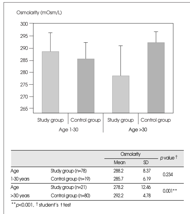
Fig. 2. A statistical significance is found when comparing patients over 30 years of age.
