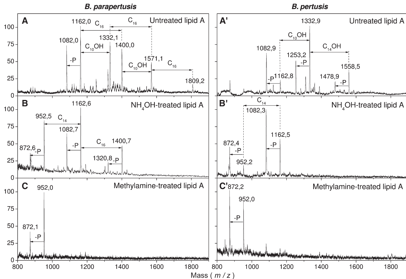
Fig. 2. Matrix-assisted laser-desorption/ionisation mass spectrometry of: B. parapertussis lipid A NRCC4323 (A); lipid A obtained after a first primary deO-acylation step (at 50°C for 5 h with ammonium hydroxide) (B); lipid A obtained after complete deO-acylation (at 37°C for 5 h with methylamine) (C). A', B', C': same treatments for B. pertussis strain 1414 lipid A.
