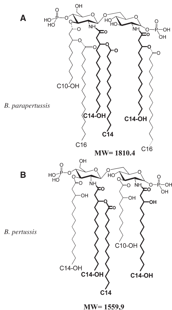
Fig. 3. Structures corresponding to the higher mass molecular species present in the negative-ion spectra of B. paraptentussis (A) and B. pertussis (B). Dotted lines indicate incomplete fatty acid substitution. Bold lines represent common fatty acids in both lipid A structures.
