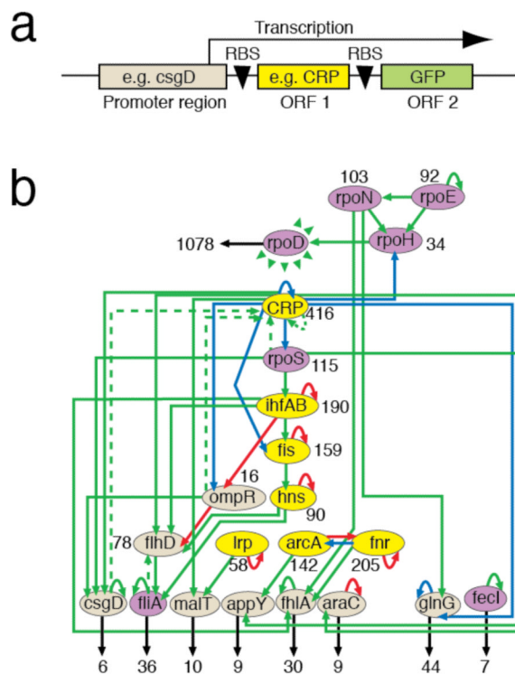
Figure 1. Promoter-ORF network rewiring
