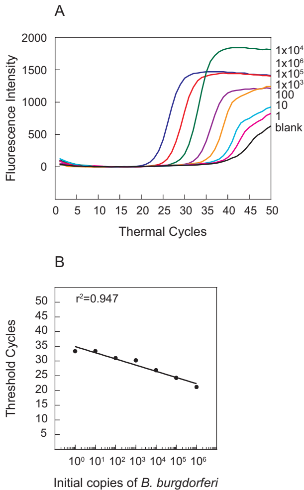
Figure 3 SYBR Green I, a non-specific double stranded nucleotide fluorescent probe, can detect a wide range of B. burgdorferi numbers in the presence of mouse DNA. The amplification plots (A) show PCR of the recA gene of B. burgdorferi strain N40 as detected by SYBR Green at the end of each PCR cycle. Uninfected mouse joint DNA (containing 10 5 nidogen copies) spiked with a ten-fold dilution of B. burgdorferi DNA, starting with 10 6 spirochete copies, was used for this assay. A standard curve (B) and a direct correlation (r 2 = 0.947) between Ct number and B. burgdorferi number shows that a wide range of spirochete numbers can be detected in our system using SYBR Green.
