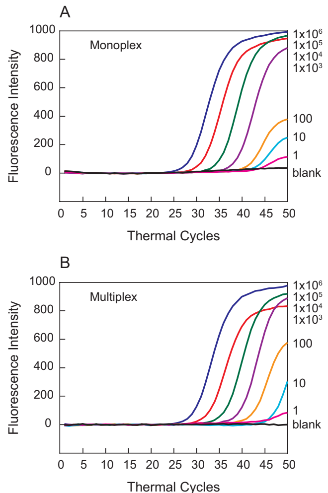
Figure 5 Multiplex analysis does not affect sensitivity of detection of B. burgdorferi by molecular beacons. A comparison of monoplex (A) and multiplex (B) assay systems of different dilutions of B. burgdorferi spiked in the mouse DNA containing 10^5 nidogen copies indicates that multiplex analysis does not affect the sensitivity of spirochete detection.
