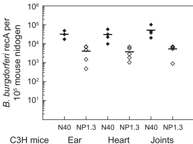
Figure 6 Multiplex analysis of mouse infected tissues using molecular beacons indicate that bgp -defective mutant, NP1.3, is less efficient in tissue colonization than the wild-type N40 strain. Number of B. burgdorferi strain N40 (filled diamonds) or NP1.3 (open diamonds) present in different tissues at two weeks of infection of C3H/HeN mice were determined by qPCR using molecular beacons. The spirochete load was normalized to 10 5 nidogen copies. After determination of the Ct values for recA of B. burgdorferi and mouse nidogen in the PCR assays, the standard curve (Figure 2B) was used to determine the number of spirochetes per 10 5 nidogen copies (~6 × 10 4 cells) of the infected mouse tissues.
