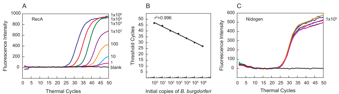
Figure 2 Molecular beacons can detect B. burgdorferi between 1 and 10^6 in multiplex assay, when C3H mouse DNA was also included. Amplification plots of recA and nidogen genes in PCR assays to estimate quantities of B. burgdorferi (A) and mouse (C) DNA are shown. Uninfected mouse heart DNA (containing 10^5 nidogen copies) spiked with ten-fold dilutions of B. burgdorferi strain N40 ranging from 1 to 10^6 were used in the PCR assays containing both RecA3 and Nidogen molecular beacons. Sensitivity and specificity of the detection system is indicated by the ability of RecA3 and Nidogen molecular beacons to quantify the amplicons from both the recA and the nidogen genes in the same PCR assay tubes. A high coefficient of correlation ( r^2 = 0.996 ) between the Ct values and the spirochete number obtained from the standard curve (B) indicates that the molecular beacons can be used effectively to quantify spirochete burden in infected tissues using multiplex assay system.
