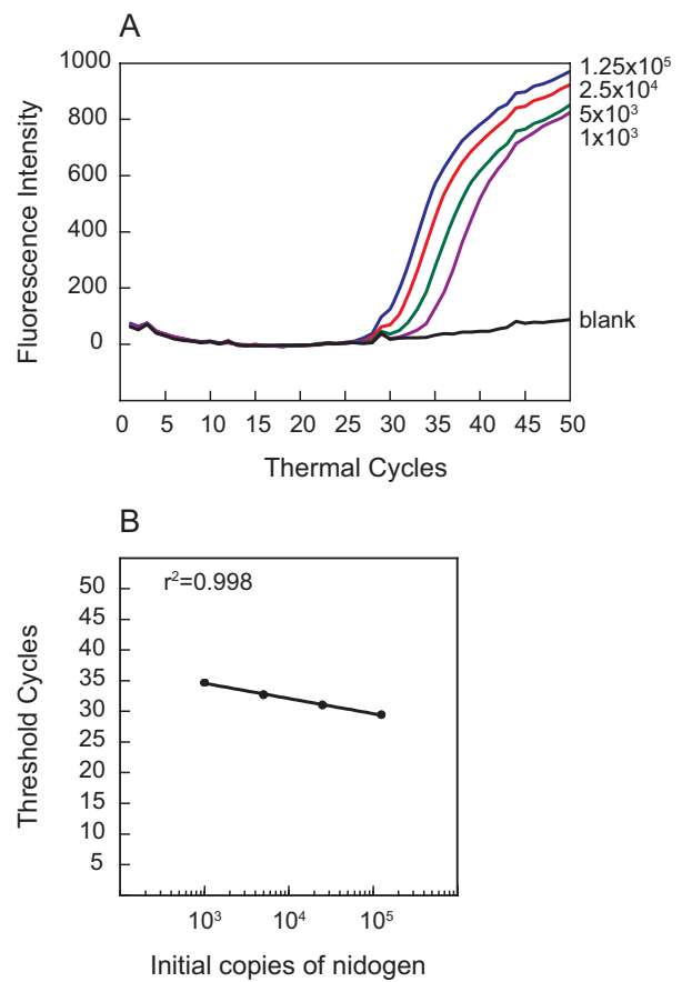
Figure 4 A serial dilution of mouse joint DNA is detectable by Nidogen molecular beacons. Amplification plots of five-fold dilution of mouse DNA used in PCR assays with Nidogen molecular beacon for detection of nidogen amplification products are shown (A). A standard curve (B) and high coefficient of correlation (r 2 = 0.998) indicates that the Nidogen molecular beacon is effective in detecting 200 ng to the low level (1 ng) of mouse DNA.
