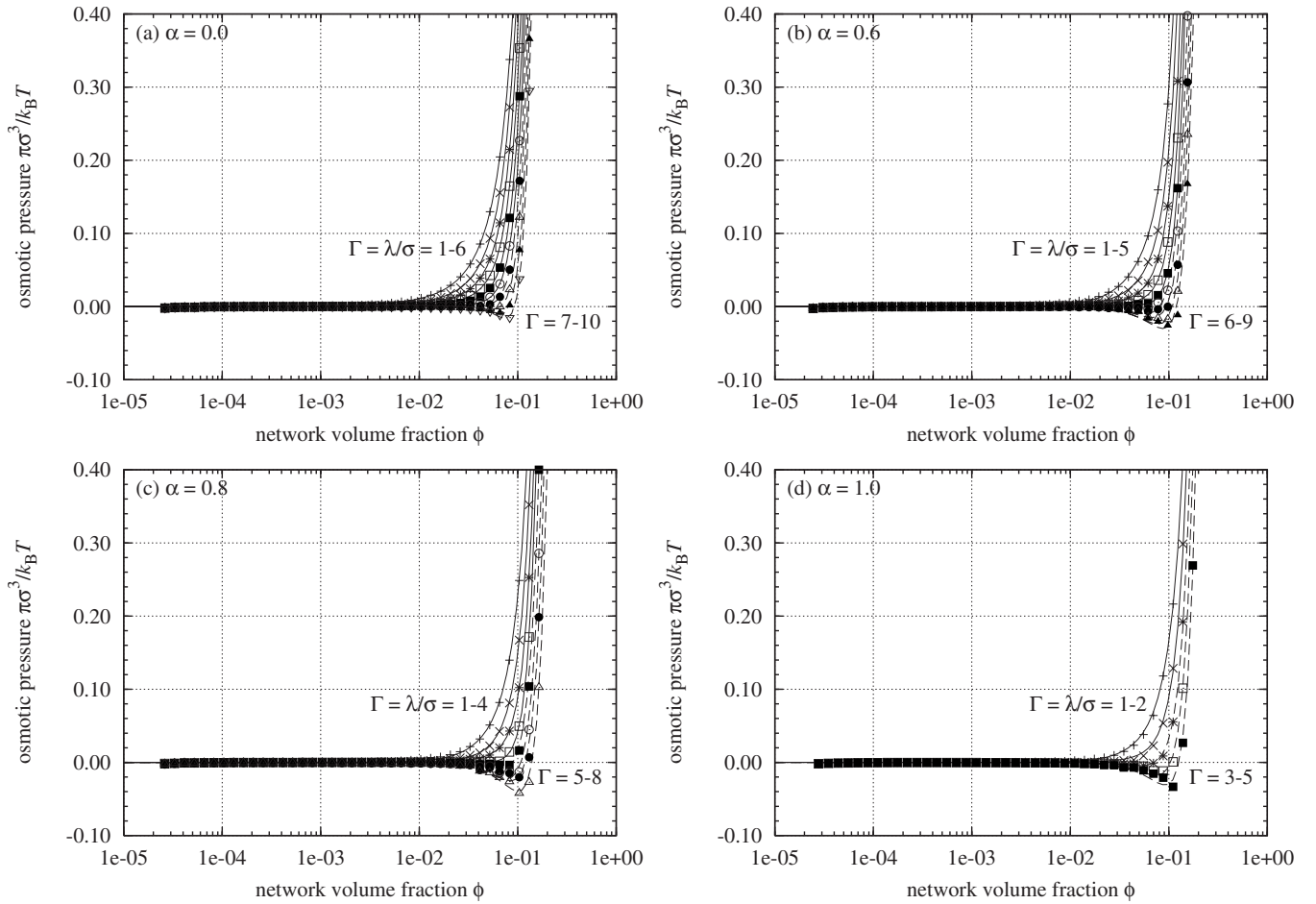
FIG. 4. Osmotic pressure of simulated polyelectrolyte gels. The curves are obtained by fitting Eq. (2) to the data via Eq. (20).
