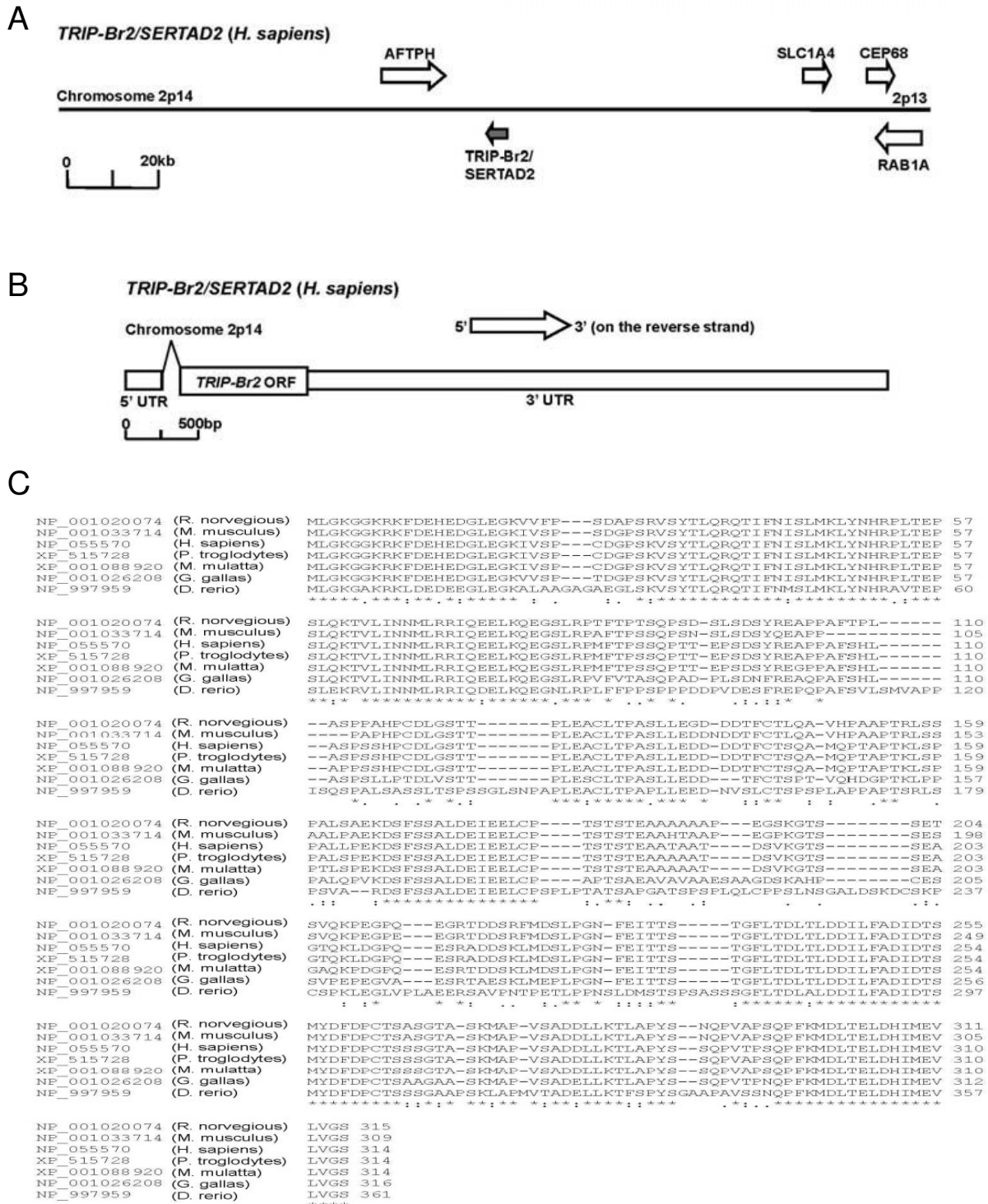
Figure 1 Gene structural organization of human TRIP-Br2. (A) TRIP-Br2 is localized at chromosome 2p14 of the human genome (B) TRIP-Br2 consists of two exons that are separated by an intron encoding splice donor-acceptor (GT-AG) sequences at either end. (C) Multiple sequence alignment of TRIP-Br2 proteins from widely divergent species by BLAST/ClustalW analyses.
