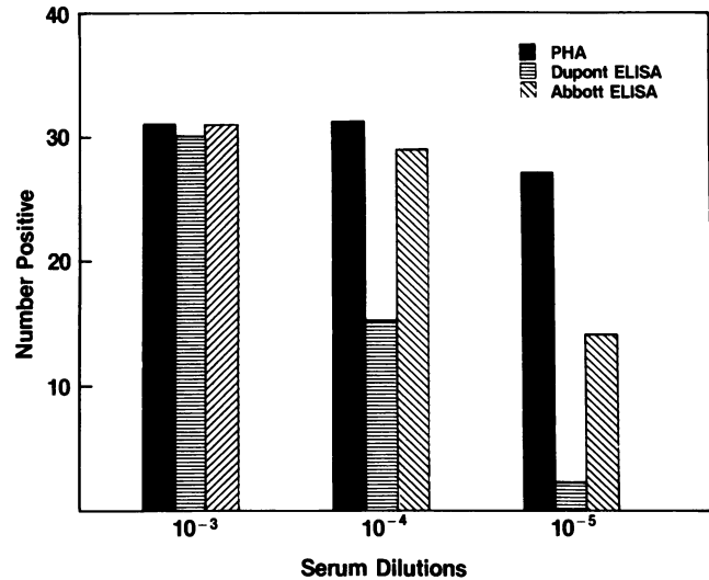
FIG. 2. Comparison of sensitivities of PHA, Dupont ELISA, and Abbott ELISA. Serum samples that remain positive by each test at 10^{-3} , 10^{-4} , and 10^{-5} dilution are compared.
