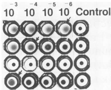
FIG. 1. Representative titration pattern of sera by PHA. Arrows indicate the highest dilution of serum giving a positive agglutination pattern. The sample in row 3 (from the top) is a negative serum. The last well in each row (control) contains a 10^{-3} dilution of the respective serum to which RBC coupled with bovine serum albumin are added.
