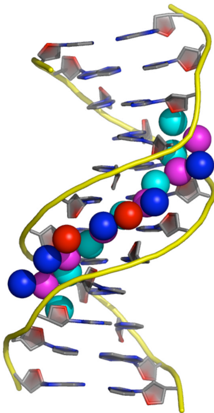
Figure 3. Narrow minor groove and multilayer spine of hydration in a poly(dA:dT) tract Shown is a representation of the atomic resolution X-ray crystallographic structure of [d(CGCAAATTTGCG)] 2 [**44]. The DNA backbones are shown as yellow curves, with the bases shown in a partial-charge-coded stick representation. The narrow minor groove of the A 3 T 3 stretch has many high occupancy water molecules, 4 layers deep, shown here as spheres, color coded according to their layer from innermost to outermost as cyan, purple, blue, and red, respectively. The multiple layers, extensive hydrogen bonding, and high occupancy of these waters all suggest that they may have strongly favorable energetic interactions with themselves and the DNA. Figure kindly provided by Prof. L.D. Williams (Georgia Tech.).
