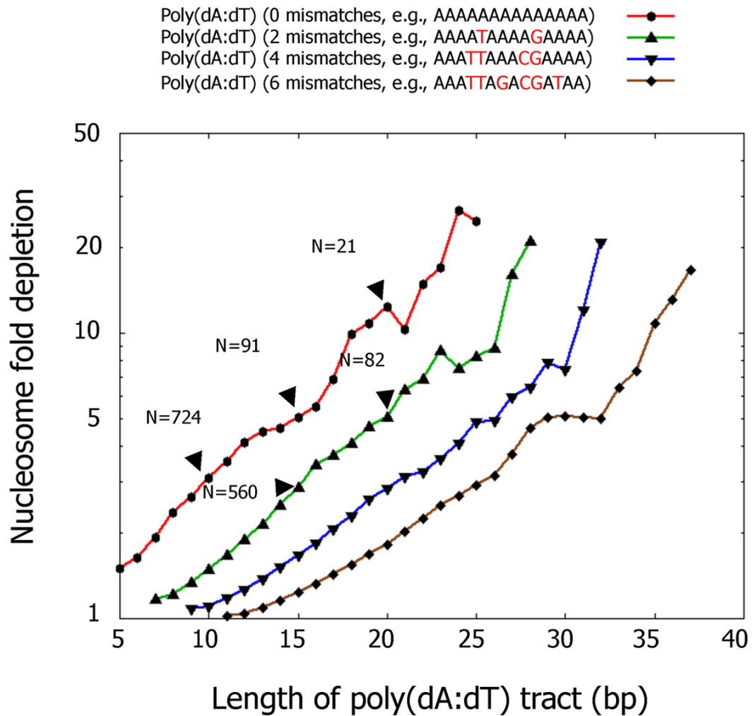
Figure 1. Nucleosome are relatively depleted over poly(dA:dT) tracts in vivo
