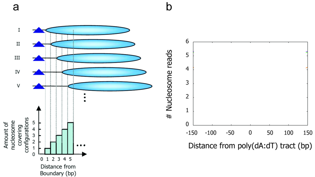
Figure 2. Poly(dA:dT) tracts create larger nucleosome-depleted regions
