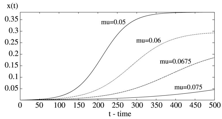
Fig. 6. The plots of the proportion of infective humans in the delayed Ross–Macdonald model (1) when the per capita mortality rate of the mosquito increases from \mu = 0.05 per day to \mu = 0.075 per day.
