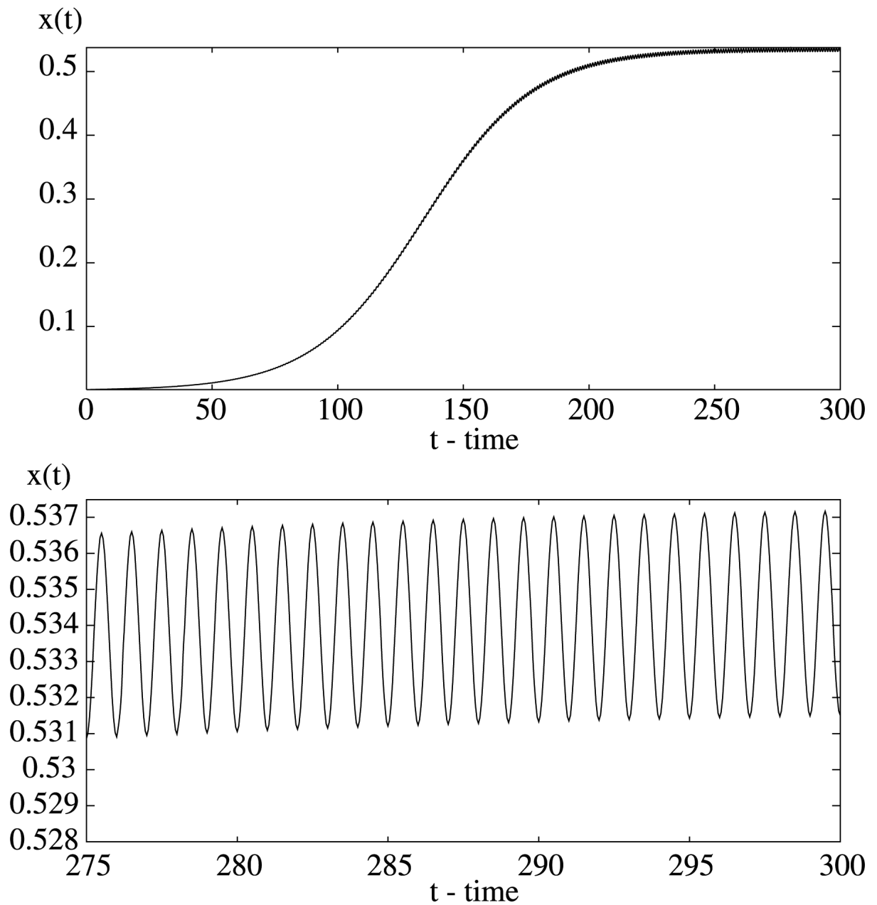
Fig. 7. The plots of the proportion of infective humans in the delayed Ross–Macdonald model (1) when the number of mosquitoes per human host is a periodic function, m(t) = p + q \sin(2\pi t) with p = 1.5 and q = 1 .
