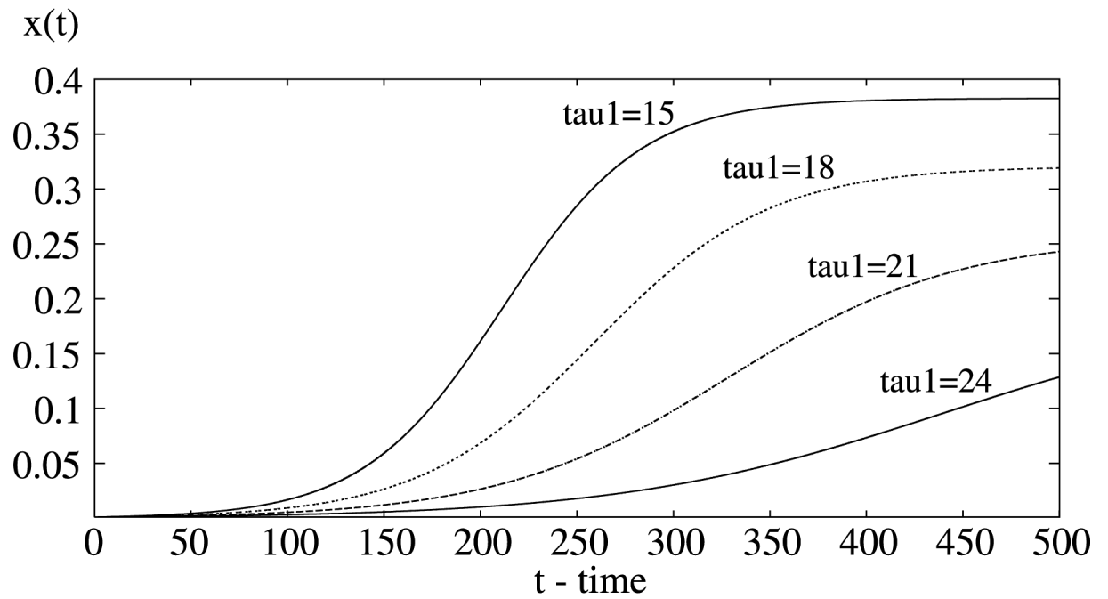
Fig. 3. In the delayed Ross–Macdonald model (1), increasing in the incubation period in the human will decrease the proportion of infective human population. Here \tau_1 increases from 15 days to 24 days.
