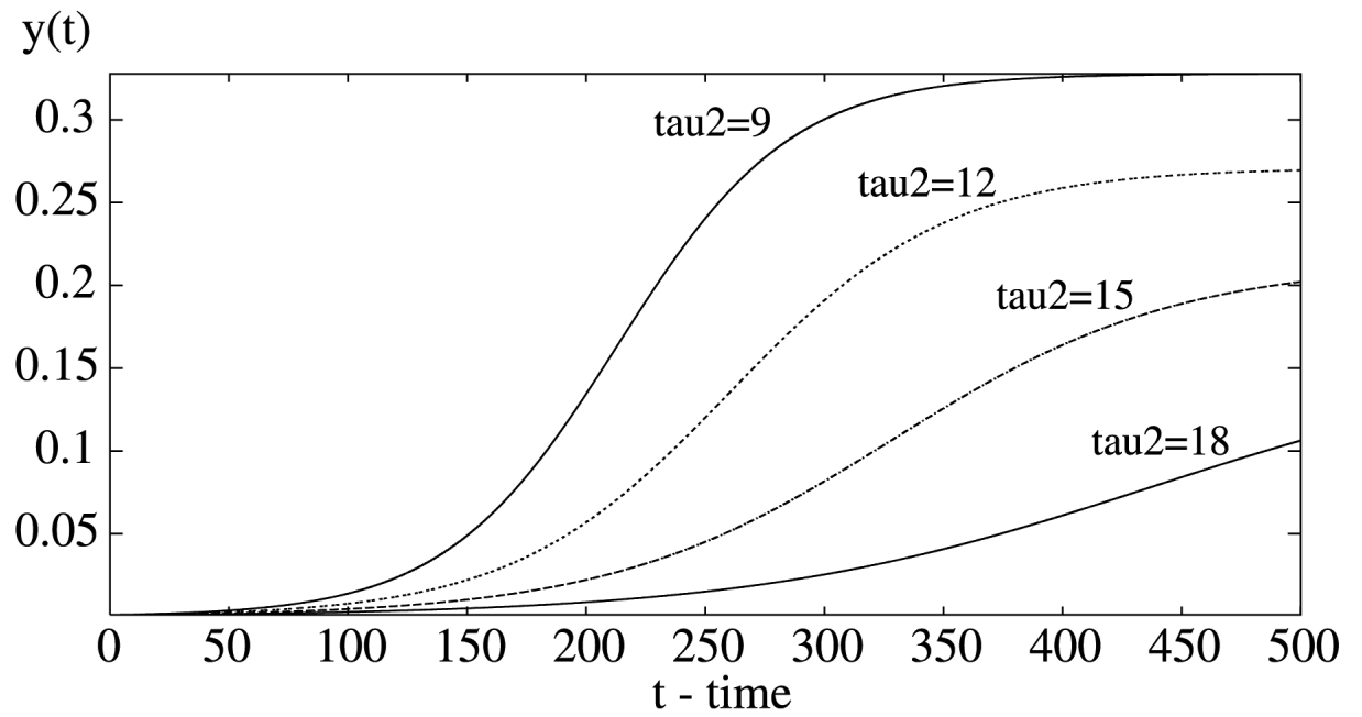
Fig. 4. In the delayed Ross–Macdonald model (1), increasing the incubation period in the mosquito can also decrease the proportion of infected mosquito population. Here \tau_2 is increased from 9 days to 18 days.
