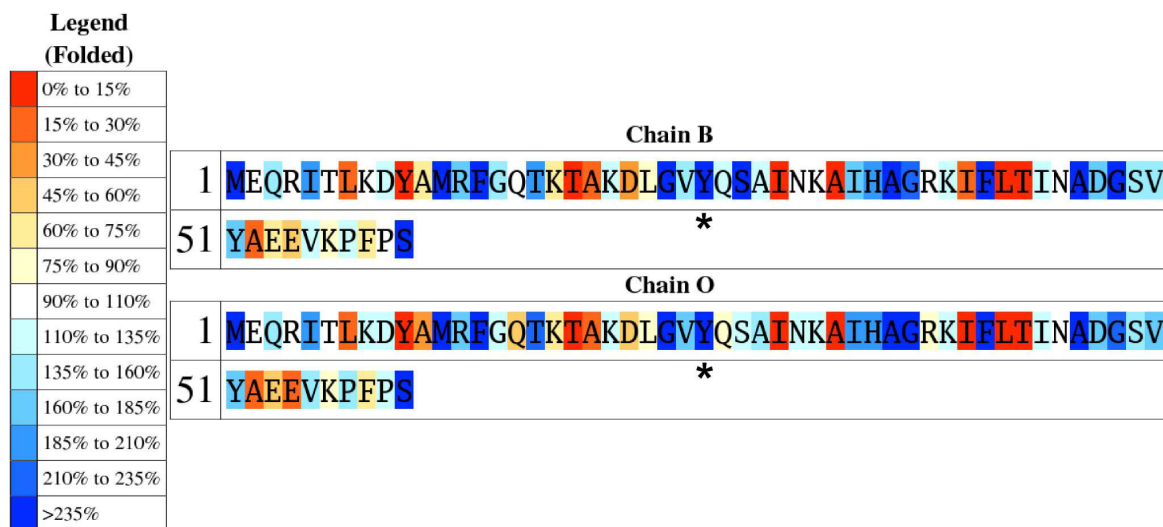
Figure 3 Colour-coded sequence for the folded SASA of [PDB:5cro], calculated with ProtSA. The specific degree of burial in the folded state of a given residue type varies widely. Tyr 26 is clearly more exposed than the average tyrosine residues present in the test set of 11 proteins (see text), which could be suggestive of a possible 'reverse hydrophobic effect'. This effect can be discarded by inspection of figure 4a. The data shown is for 1.4 Å of solvent radius and 2000 conformations. Tyr 26 is labelled.
