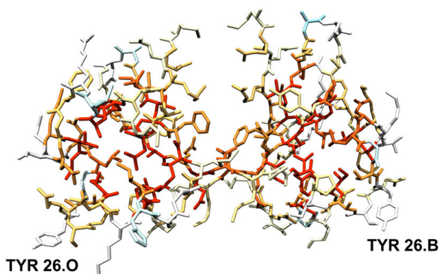
Figure 5 X-ray structure of [PDB:5cro] colour-coded by the ratio of folded SASA over unfolded SASA. Colour-code is as in the legend of figure 4. Tyr 26, labelled in white colour, indicating that its solvent exposure in the folded state is very similar to that in the unfolded ensemble.
