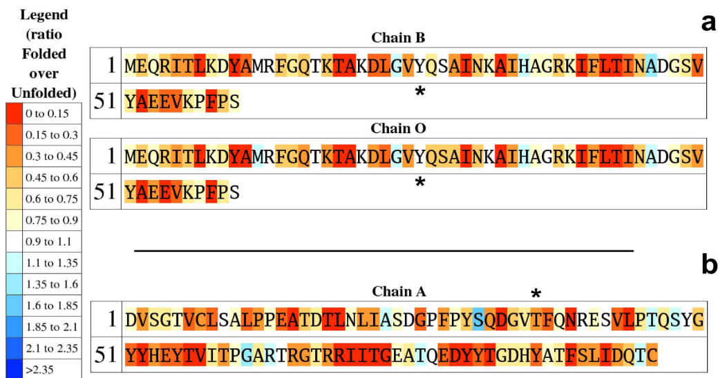
Figure 4 Colour-coded sequences of the ratio of folded and unfolded SASA for [PDB:5cro] and [PDB:1ucj]. Upon folding, most residues tend to be less exposed to solvent than in the unfolded state, as shown by the majority of reddish residues in the figure. However, some residues may be more exposed in the folded state (bluish residues). a) Tyr 26 (labelled) of [PDB:5cro] has a ratio of folded SASA over unfolded SASA in the range 0.9–1.1, suggesting that no reverse hydrophobic effect is taking place (see text). b) Thr 36 (labelled) of [PDB:1ucj], as most residues, is also in a reddish shade. Since this residue bears a polar side chain, its burial is suggestive of a destabilizing contribution to the native conformation. The data shown in both cases is for 1.4 Å of solvent radius and 2000 conformations.
