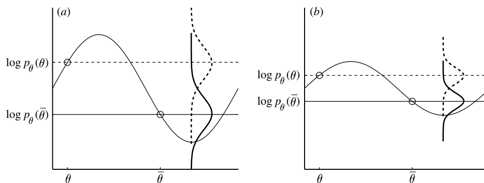
Figure 5. The discrimination parameter \sigma is undetermined. (a) Graph of an example log prior, \log p_\theta(\theta) (solid horizontal sinusoid curve), as a function of lighting direction \theta . Given two hypothetical neurons with preferred lighting directions \theta and \bar{\theta} , their responses are determined by their log probability density functions, \log p(\theta) and \log p(\bar{\theta}) , indicated by the vertical dashed and solid curves, respectively. For a given stimulus, the larger of the two observed values from the probability density functions \log p(\theta) and \log p(\bar{\theta}) determines the lighting direction assumed by the observer, and this, in turn, determines the concave/convex observer response. These two observed values are noisy estimates of the probability density function means, so the choice probability q (see equation (2.19)) is determined by the relative overlap of the probability density functions (vertical dashed and solid curves) for these two quantities. (b) A log prior with amplitude variations k times smaller than in (a) leads to the same choice probabilities as in (a), provided the noise level \sigma is also reduced by a factor k . (For simplicity, this analysis assumes a concavity preference of 0.5.)
