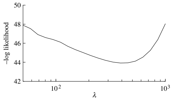
Figure 3. Cross-validation. Result for estimating the value of the smoothing parameter \lambda for observer a in figure 4, with \sigma = 2 . The minimum with respect to the negative log likelihood corresponds to \lambda \approx 400 . This curve is typical of that obtained for other observers, and a value of \hat{\lambda} = 400 was therefore used for all human observers.
