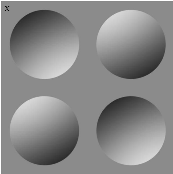
Figure 1. Typical stimulus presented to an observer on a single trial. The observer’s task is to indicate whether or not the quadrant marked with a cross (X) appears convex or concave. This response implicitly defines the perceived direction of the light source. For example, if the marked quadrant is perceived as convex, then this implies that the light originates from the lower right (i.e. approx. 300°), but if it is perceived as concave, then this implies that the light originates from the upper left (i.e. approx. 120°).
