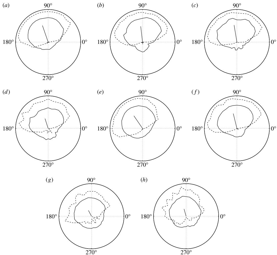
Figure 4. Polar plots of estimated priors for eight observers. Each graph shows the frequency of convex responses (dashed) as a function of light-source direction. This is essentially a sample from the observer's posterior, and is used to estimate the prior (solid). For display purposes, the lengths of all mean vectors (solid line) have been scaled by the same factor across all graphs, and all graphs are drawn to the same scale (see appendix C). Note that all biases are to the left, with values of 20°, 7°, 9°, 18°, 34°, 14°, 28° and 16°, respectively (mean 18°). These results were obtained using all the data for each observer with \lambda = 400 and \sigma = 2 .
