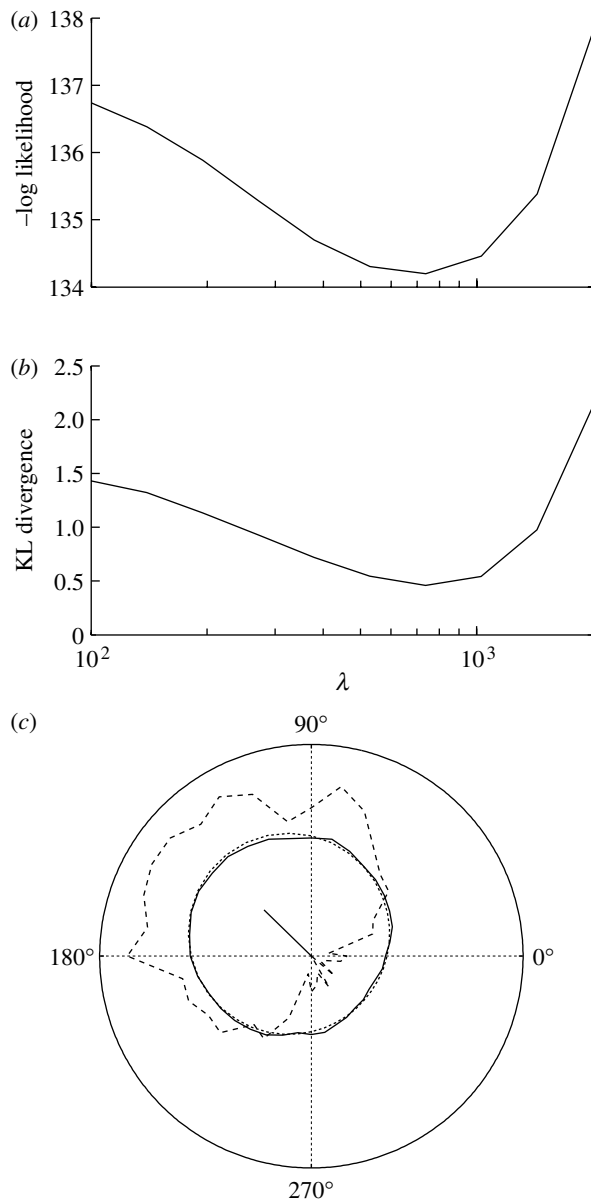
Figure 2. Evaluating cross-validation method for estimating the value of the smoothing parameter \lambda . Results for the simulated observer's data shown in (c) for \sigma=1 . See appendix B. (a) At each sampled value of \lambda , three quarters of the data were used to estimate the prior. Using this prior, the likelihood of the remaining quarter was evaluated using equation (2.23), where \sigma=1 . This was repeated once for each of four disjoint quarters, and the mean of the four resultant likelihood functions is plotted here. The minimum with respect to the negative log likelihood corresponds to \lambda \approx 700 . (b) To evaluate the success of cross-validation for each sampled value \lambda_j of \lambda , the Kullback–Leibler (KL) divergence between the known prior p_\theta^*(\theta) of this simulated observer and the prior \hat{p}_\theta(\theta) obtained with \lambda_j was calculated as E_{\text{KL}} = 1000 \times \Delta\theta \sum \hat{p}_\theta(\theta_i) \log \hat{p}_\theta(\theta_i) / p_\theta^*(\theta_i) , where i = (0, 10, \dots, 350) , \theta_i = 10 \times i and \Delta\theta = 10^\circ . The minimum with respect to the KL distance also corresponds to \lambda \approx 700 , confirming that cross-validation chooses a value of \lambda , which provides a good estimate of the true prior. (c) Estimating the light-from-above prior p_\theta(\theta) for a simulated observer. The lighting direction varies around the circle, and the probability that the stimulus was judged to be convex varies with distance from the origin. The graph shows (i) a sample from the posterior p(c_0|\mathbf{x}) as the proportion of convex responses (dashed), (ii) the known prior (dotted), (iii) the estimated prior (solid), based on the proportion of convex responses, as it
