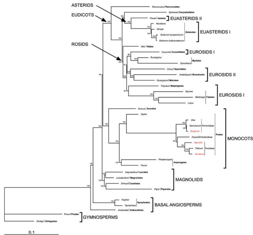
Fig. 6. Phylogenetic tree of 38 taxa based on 61 plastid protein-coding genes using maximum likelihood. The tree has a ML value of -\ln L = 348086.2268 . Numbers at nodes are bootstrap support values 50%. Ordinal and higher level group names follow APG II (2003). Taxa in red are the new genomes reported in this paper
