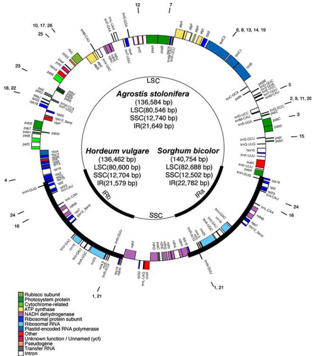
Fig. 1. Gene map of Hordeum vulgare , Sorghum bicolor and Agrostis stolonifera chloroplast genomes. The thick lines indicate the extent of the inverted repeats ( IRa and IRb ), which separate the genome into small ( SSC ) and large ( LSC ) single copy regions. Genes on the outside of the map are transcribed in the clockwise direction and genes on the inside of the map are transcribed in the counterclockwise direction
