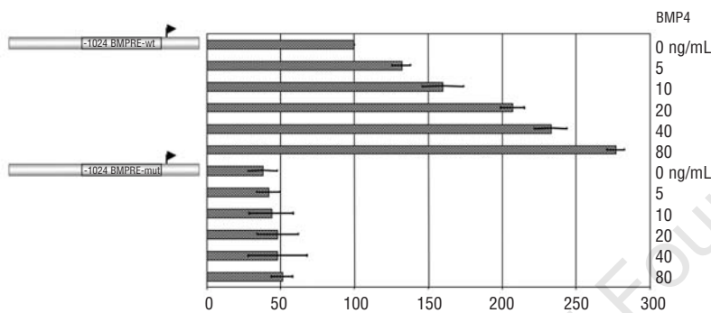
Figure 2. The -1024 BMPRE-wt Hep/Luc but not the mutated constructs responds in a dose-dependent manner to BMP4. HepG2 cells were transfected with the -1024/BMP-RE wt or mutated and were treated with increasing amount of BMP4.
