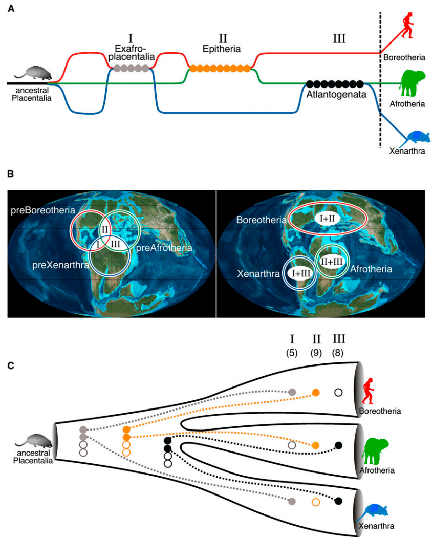
Figure 4. Hypothetical scenarios of interspersed ancestry of placentals. (A) Hybridization/introgression scenario: Initially, the three placental lineages diverged and separated from an Eomaia -like ( Eomaia scansoria ) common ancestor. Alternate gene flow between the lineages led to a mosaic pattern of relationships among the current species. The sequence of genetic flow leading to significant support for Exafroplacentalia, Epitheria, and Atlantogenata was chosen randomly and not meant to indicate a specific time course. The lineages leading to Boreotheria, Afrotheria, and Xenarthra are shown in red, green, and blue, respectively. Gray circles represent diagnostic retroposon insertions for Exafroplacentalia, orange circles for Epitheria, and black circles for Atlantogenata. (B) Geographic transitions at the time of separation of the three lineages during the Cretaceous. (Left terrestrial globe) Possible overlapping geographical distribution of the three placental lineages before continental drift, the expected period of genetic flow between the lineages; (right terrestrial globe) separation of the continents and divergence of placental lineages possibly prohibiting further gene flow (Murphy et al. 2001b; Wildman et al. 2007). Roman numerals indicate exchanges of genetic material between the species shown in A. (C) Randomly sorted ancestral alleles: Fixation of retroposon alleles was not completed in the ancestral population before the separation of lineages. After the proliferation of inserted retroposon alleles, the distributions to different lineages occurred randomly (broken lines). After fixation of the alleles in the terminal lineages, a mosaic pattern of relatedness remains. (I) Five orthologous markers represent Exafroplacentalia, (II) 9 markers (plus an additional marker previously described in Kriegs et al. 2006 that was undetected here) represent Epitheria, and (III) 8 markers represent Atlantogenata. Open circles represent alleles without retroelements.
