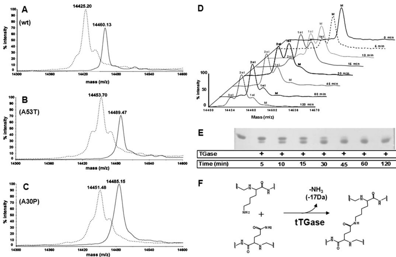
FIGURE 2. tTG-catalyzed cross-linking of \alpha -syn involves one to three intramolecular cross-links. A–C, MALDI-TOF/TOF analysis of native (—) and cross-linked (---) \alpha -syn, showing that most tTG-catalyzed cross-linking products of WT or disease-associated mutant forms of \alpha -syn are intramolecularly linked (predominant peak with two cross-links), and up to three intramolecular cross-links can occur ( left shoulder ). The abbreviations M and m/cl are used to designate native and cross-linked \alpha -synuclein, respectively. D and E , kinetic analysis of \alpha -syn (A30P) cross-linking monitored by MALDI-TOF and SDS-PAGE. F , schematic depiction of the tTG-catalyzed chemical reaction (isodipeptide formation) between glutamine and lysine residues.
