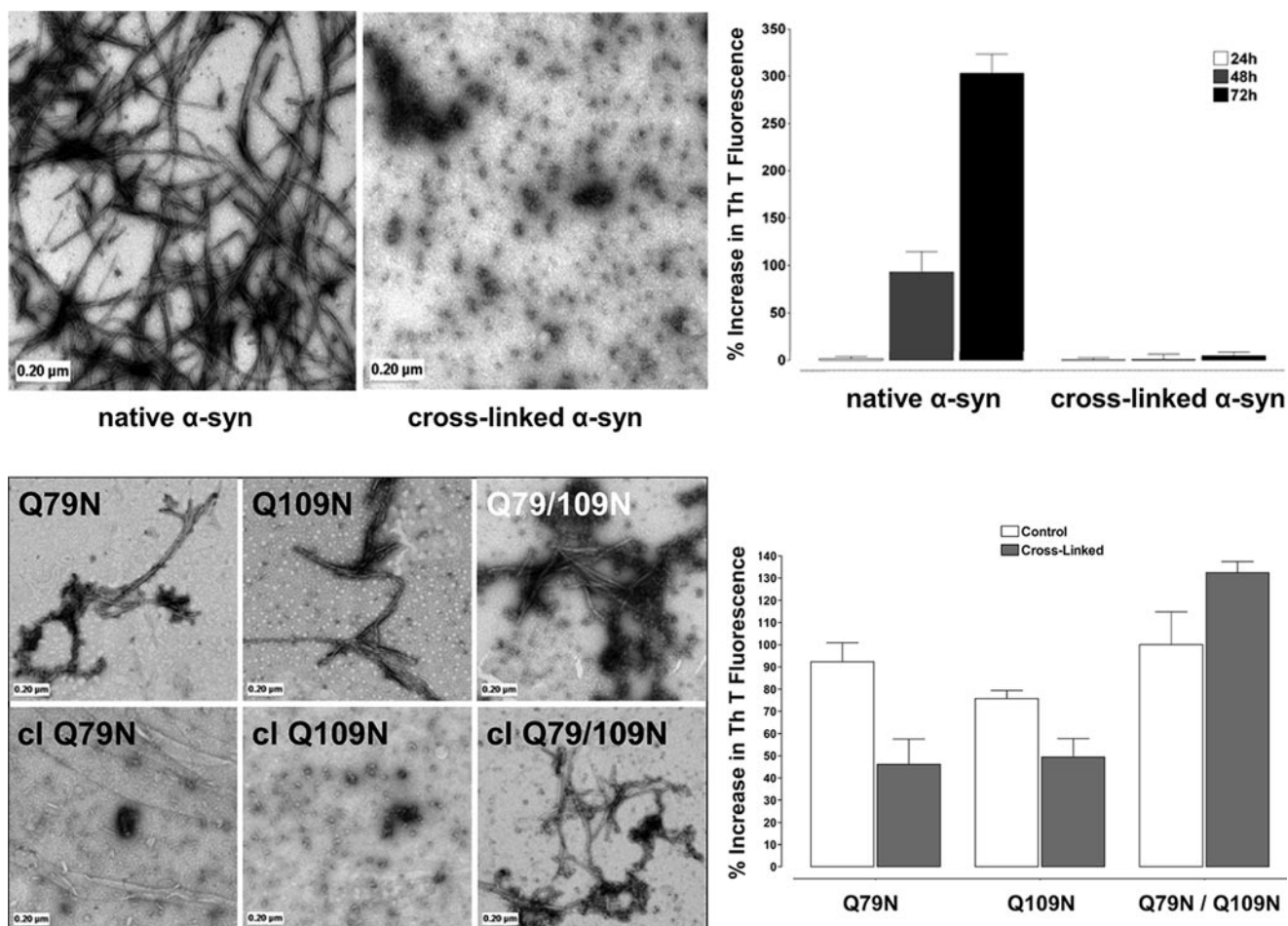
FIGURE 7. tTG inhibition of \alpha -syn fibrillization is mediated by intramolecular cross-linking that involves residues Gln 79 and Gln 109 . Negatively stained TEM images (scale bar, 0.2 \mu m) and the corresponding ThT fluorescence of native and cross-linked A53T (upper panels) and Gln to Asn \alpha -syn mutants (Q79N, Q109N, and Q79N/Q109N; lower panels) after 3–4 days of incubation under fibril-forming conditions. The ThT values are the mean \pm S.D. of three independent measurements. cl , cross-linked.
