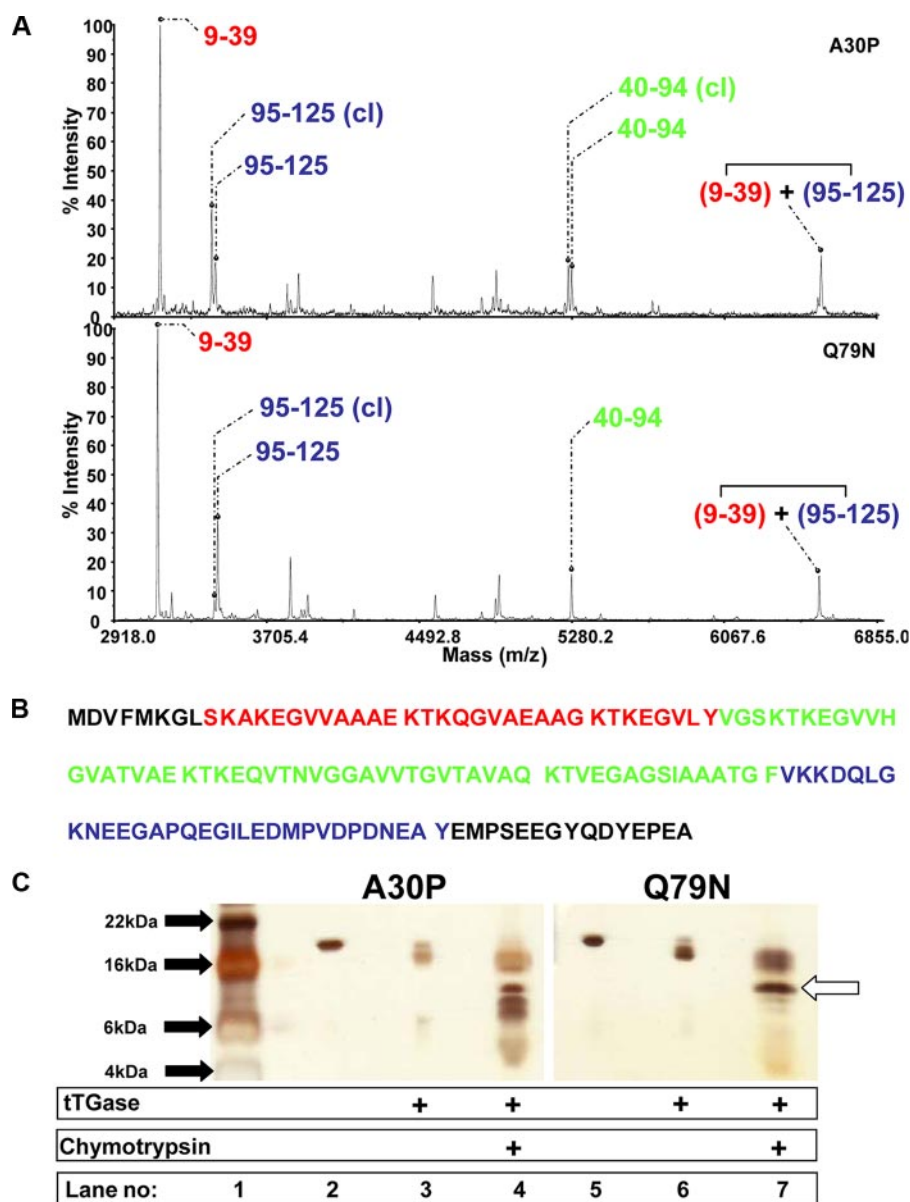
FIGURE 3. MALDI-TOF/TOF analysis of chymotrypsin-digested cross-linked Q79N mutant \alpha -syn. Proteolytic digestion of cross-linked A30P (A, upper spectrum) and cross-linked Q79N \alpha -syn (A, lower spectrum) yields a large fragment with masses of average m/z 6558.12 [M + H]^+ and 6534.47 [M + H]^+ , respectively, which is explained by a cross-link between fragments 9–39 and 95–125. The difference in mass observed with these cross-linked fragments accounts for the presence of a proline residue in A30P \alpha -syn. B, proteolytic fragments of \alpha -syn generated by chymotrypsin. C, silver-stained SDS-PAGE of chymotrypsin digests, showing a large fragment (white arrow) that appears to be resistant to further digestion, which may account for the cross-linked fragments involving residues 9–39 and 95–125.
