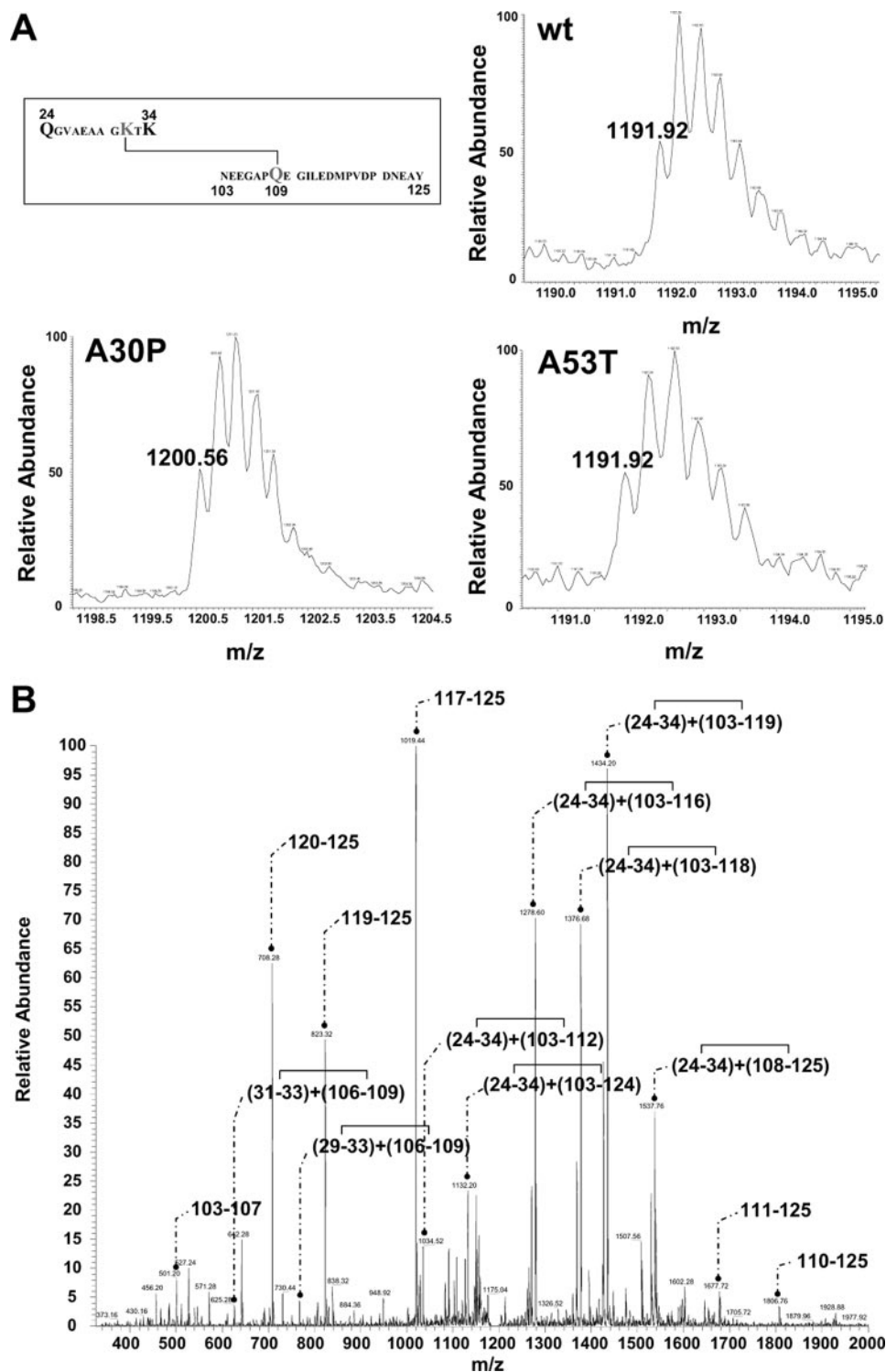
FIGURE 5. tTG-mediated cross-linking of residues Gln 109 to Lys 32 . A , ESI-MS analysis of the digestion products obtained after subjecting cross-linked WT, A30P, and A53T \alpha -syn to sequential proteolysis with chymotrypsin followed by Lys-C. Lys-C fails to cleave at residue Lys 32 , suggesting that this residue is cross-linked to residue Gln 109 (inset in A ). The difference in mass observed with A30P \alpha -syn is because of the proline residue. B , ESI-MS collision-induced dissociation fragmentation of A30P \alpha -syn of the parental fragment of m/z 1191.92 [ M + 2H ] 2+ , in which the C and N termini are cross-linked together. Fragmentation of C-terminal residues 103–125 appeared more evident as compared with N-terminal residues of 24–34. Nevertheless, the smallest detectable fragment with a mass of m/z 625.28 could be associated to the N-terminal residues 31–33 cross-linked to the C-terminal residues 106–109.
