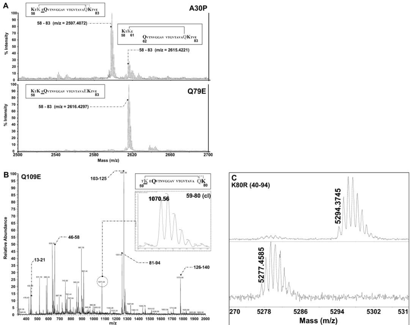
FIGURE 6. Residue Gln 79 is cross-linked to residue Lys 60 within the NAC region of \alpha -syn. A, MALDI-TOF/TOF (reflectron mode) analysis of cross-linked and digested A30P and Q79E \alpha -syn. Sequential digestion of cross-linked A30P and Q79E \alpha -syn with chymotrypsin followed by Glu-C generates a fragment of residues 58–83, with a failure to cleave at residue Glu 61 . Only fragments derived from A30P \alpha -syn appear to bear a cross-link within this region, whereas fragments from Q79E \alpha -syn no longer bear this cross-link. A small population of A30P \alpha -syn was completely digested by Glu-C, and in this case two fragments, Lys 58 –Glu 61 and Gln 62 –Glu 83 , were found to be cross-linked. B, ESI-MS analysis of cross-linked Q109E \alpha -syn followed by chymotrypsin and Lys-C digestion reveals a fragment containing residues Thr 59 –Lys 80 and an internal cross-link (inset). The incomplete cleavage at residue Lys 60 suggests a possible site of cross-linking. C, MALDI-TOF/TOF analysis (reflectron mode) of chymotrypsin-digested native K80R \alpha -syn (upper panel) and cross-linked K80R \alpha -syn (lower panel) demonstrates that cross-linking within the proteolytic fragment comprising residues 40–94 is detected, providing further evidence that residue Lys 60 serves as the primary reactive lysine residue in this particular cross-link.
