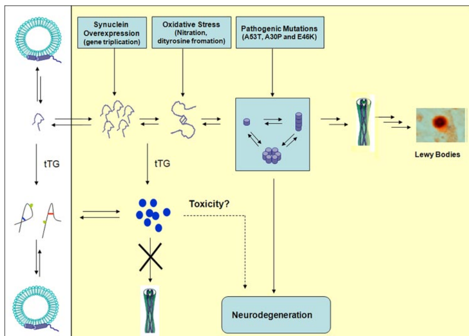
FIGURE 10. Schematic depiction summarizing our current understanding of \alpha -syn aggregation and membrane binding and how cross-linking may affect these processes. Further studies to elucidate the molecular and functional consequences of tTG-induced cross-linking of \alpha -syn in vivo are required before the exploration of therapeutic strategies based on modulating tTG levels or activity.
