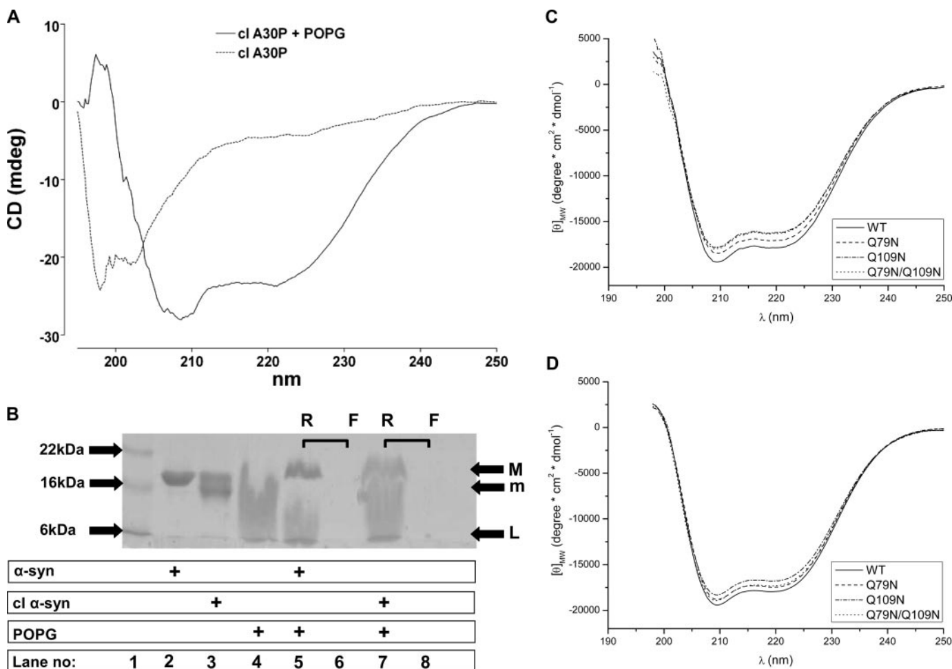
FIGURE 8. tTG cross-linking does not interfere with the binding of \alpha -syn to lipid vesicle membranes. A, CD spectra of cross-linked (cl) \alpha -syn in the presence of vesicles. In the presence of POPG vesicles, cross-linked A30P \alpha -syn undergoes a change in secondary structure from random-coil (—) to \alpha -helices (- - -). B, SDS-PAGE analysis of membrane-bound native (lane 5) and cross-linked (lane 6) monomeric \alpha -syn from A after passage through a filter with a molecular mass cutoff of 100 kDa. Both retentate (R) and flow-through (F) were separated onto a 12% SDS-PAGE (lanes 5–8; M, monomeric; m, cross-linked monomeric; L, lipids). C and D, CD spectra of membrane-bound WT and Q mutant \alpha -syn before (C) and after (D) cross-linking.
