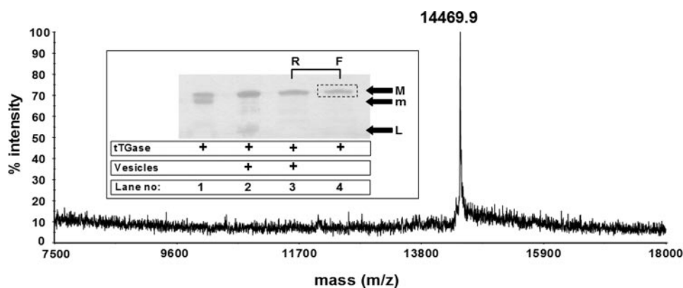
FIGURE 9. Limited tTG-mediated cross-linking of membrane-bound A30P \alpha -syn. Vesicle-bound \alpha -syn (lane 2) was dissociated from membranes by increasing the NaCl solution concentration to 300 mM. Dissociated \alpha -syn was subjected to filtration using filters with a molecular mass cutoff of 100 kDa, and the filtrate (lane 4) was analyzed by MALDI-TOF-MS. MS analysis of vesicle-bound and cross-linked \alpha -syn shows limited (only 1) cross-linking by tTG. This single cross-link does not induce the above observed shift in gel migration. The abbreviations R and F denote retentate and flow-through, respectively.
