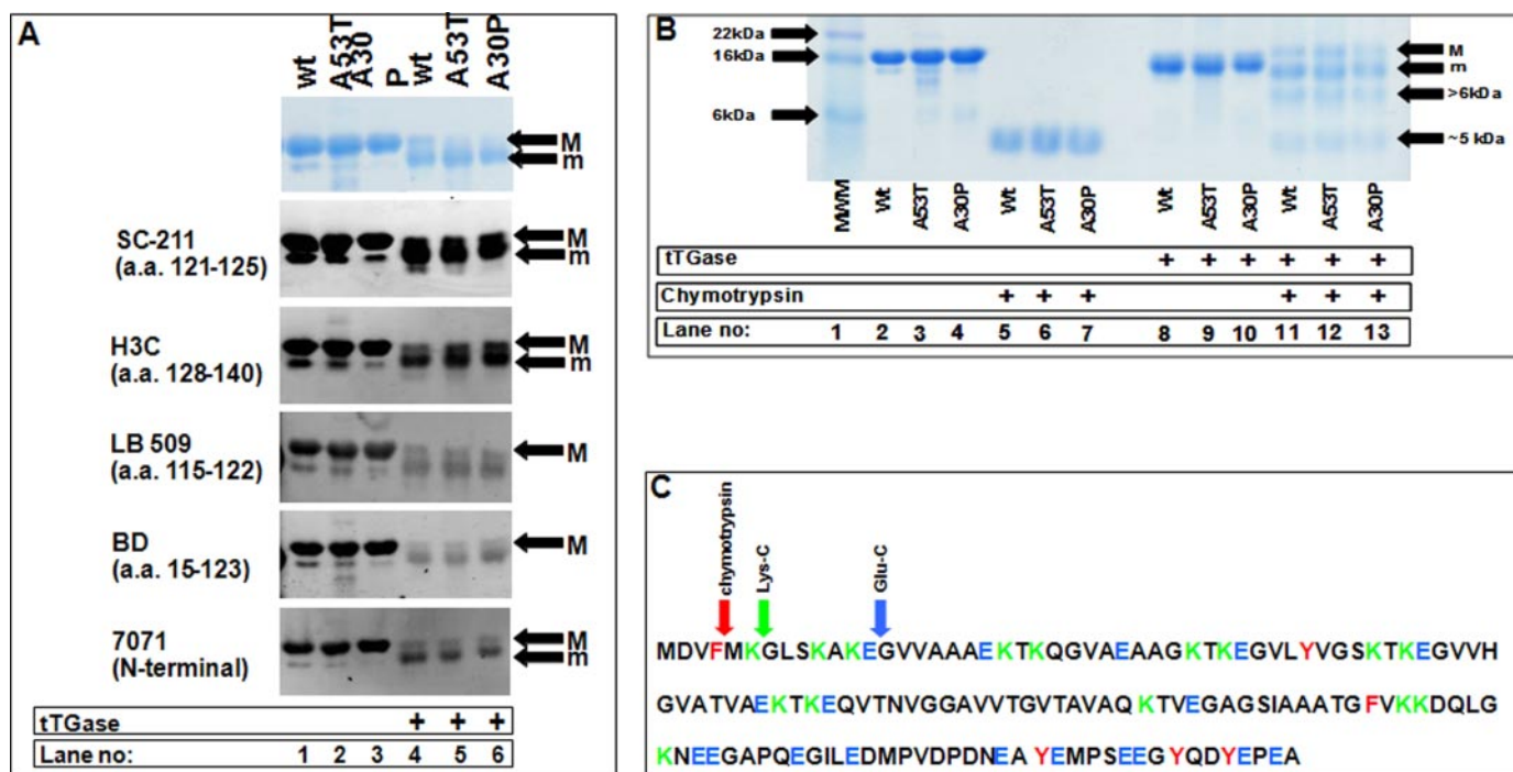
FIGURE 1. tTG-mediated intramolecular cross-linking of \alpha -syn alters its conformation, electrophoretic mobility, and accessibility to antibodies against epitopes in the N-terminal region. A , monomeric WT and mutant \alpha -syn analyzed in the absence (lanes 1–3) and presence of tTG (lanes 4–6), with the latter showing significant changes in electrophoretic mobility. The letters M and m are used to designate native and intramolecularly cross-linked \alpha -synuclein, respectively. For immunoblots, full sequence recognition was achieved for native, non-cross-linked WT and mutant \alpha -syn, using N-terminal and C-terminal monoclonal antibodies (lanes 1–3); in contrast, the N termini were not detected in cross-linked samples (lanes 5 and 6). a.a. , amino acids. B , SDS-PAGE analysis of chymotrypsin proteolysis of native (lanes 2–7) and cross-linked WT and mutant \alpha -syn (lanes 8–13). Digestion of cross-linked samples gave a pattern of proteolytic fragments (lanes 11–13) that was different from that of native \alpha -syn (lanes 5–7). C , sequence of WT \alpha -syn showing the preferred enzymatic cleavage sites of chymotrypsin (red), Lys-C (green), and Glu-C (blue).
