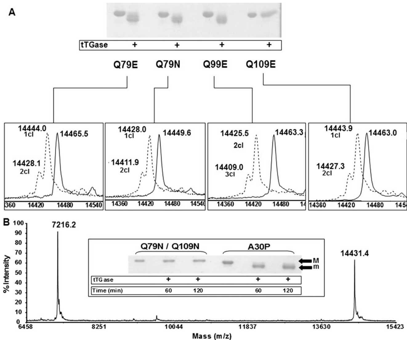
FIGURE 4. Residues Gln 79 and Gln 109 are the primary substrates for tTG-mediated cross-links. A , SDS-PAGE and MALDI-TOF/TOF analysis of tTG-mediated cross-linking of native (—) and cross-linked (---) mutants of \alpha -syn with substitutions at the putative reactive glutamine residues. B , mutating residues Gln 79 and Gln 109 to asparagine in the double mutant Q79N/Q109N abolishes tTG-mediated cross-linking of \alpha -syn, as can be seen by the unchanged, singly, and doubly charged masses of full-length protein (average m/z 14431.37 [M + H] + and 7216.18 [M + 2H] 2+ ). Inset , SDS-PAGE analysis of tTG-incubated Q79N/Q109N double mutant and A30P \alpha -syn. No shift in migration is observed with this double mutant as compared with A30P \alpha -syn. The abbreviation cl denotes cross-linked \alpha -syn.
