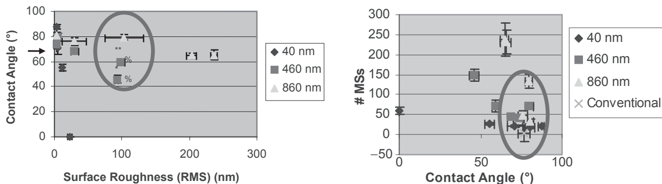
Figure 4 (Left) Changing contact angles within similar immunoassays surface roughness values; (Right) antigen capture independent of surface energetics. (Left) Circle highlights different surface energetics at the 100-nm surface roughness regime due to similar roughness values (RMS) but altered contact angles. The conventional surface contact angle, indicated by an arrow, was 76.67 \pm 3.52^\circ . Results showed that the 40-nm particle surface decreased contact angles at the highest rate ( -3.9203^\circ/\text{nm} ), the 460-nm particle surface decreased at an intermediate rate ( -0.2542^\circ/\text{nm} ), and the 860-nm particle surface decreased at the slowest rate ( -0.0661^\circ/\text{nm} ). Data = mean \pm SEM.
