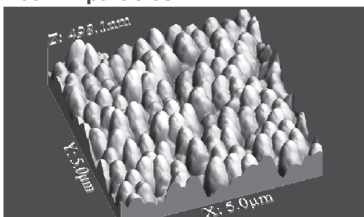
Figure 2 3D AFM images of immunoassay surfaces. AFM 3D surface images with physisorbed antibody concentrations of 11.1 \mu\text{g}/\text{mL} obtained using tapping mode in air on (A) a conventional 96-well polystyrene plate alone, (B) 40-nm gold nanoparticles conjugated with Protein A attached to a 96-well plate, (C) 460-nm polystyrene particles conjugated with Protein A attached to a 96-well plate, and (D) 860-nm polystyrene particles conjugated with Protein A attached to a 96-well plate.
