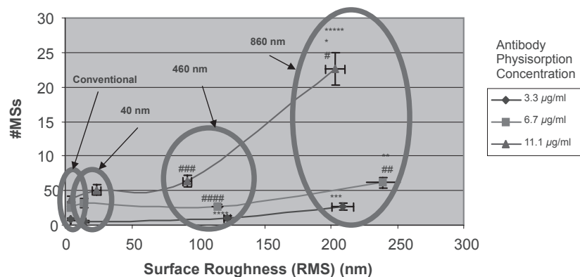
Figure 6 Increased specific antigen capture with greater surface roughness and greater physisorption of antibodies. Surface types are at stock (1:0) levels. Each circle represents similar surface types with different physisorbed antibody concentrations. A disproportionate increase in specific antigen capture was seen with respect to greater surface roughness and physisorbed antibody concentrations. Specific antigen capture at antibody physisorbed concentrations of 11.1 µg/mL increased by approximately 540% when the surface roughness (RMS) increased by approximately 1900% (that is, going from conventional or polystyrene alone surfaces to those with 860 nm particles). Data = mean \pm SEM.
