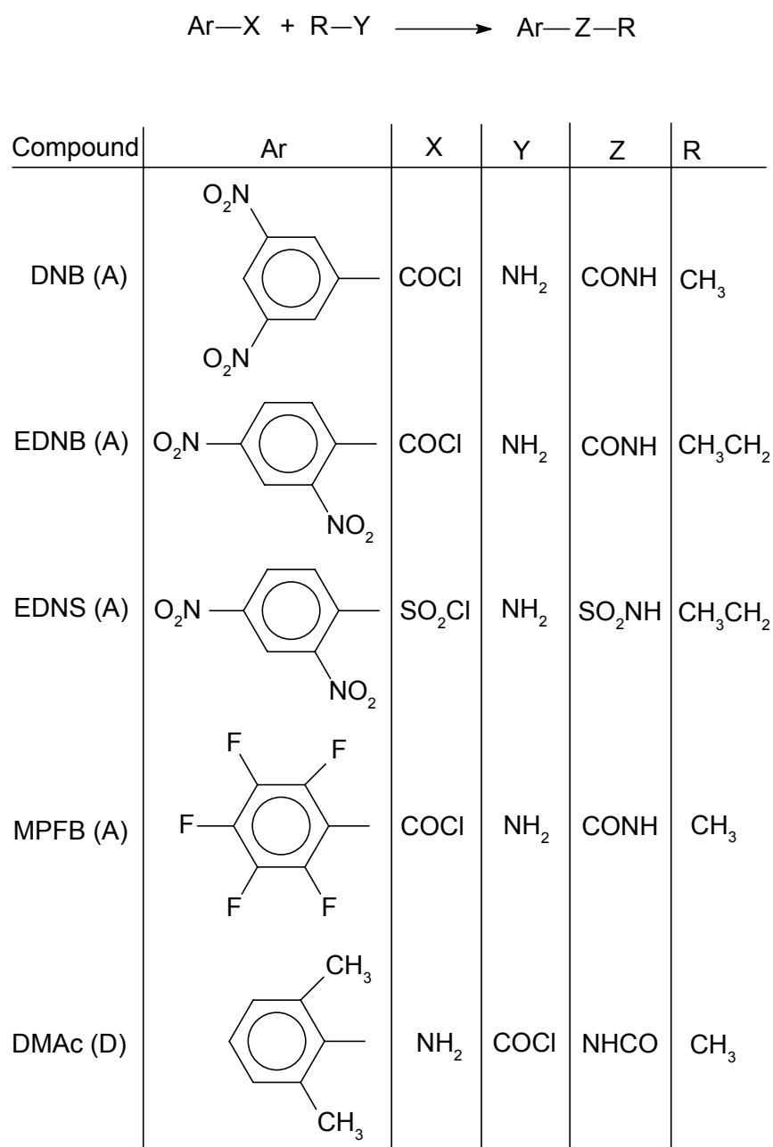
Figure 1 Synthesis and structures of acceptor (A) and donor (D) molecules studied.
