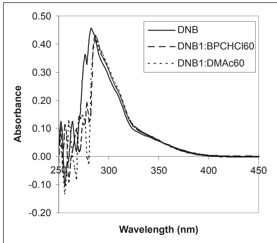
Figure 4 UV-Vis spectrum of DNB in the absence of donor-unbroken line; in the presence of BPC-dashed line; and in the presence of DMAc-dotted line. Molar ratio A:D = 1:60. Solvent, 50/50 water/acetonitrile.
