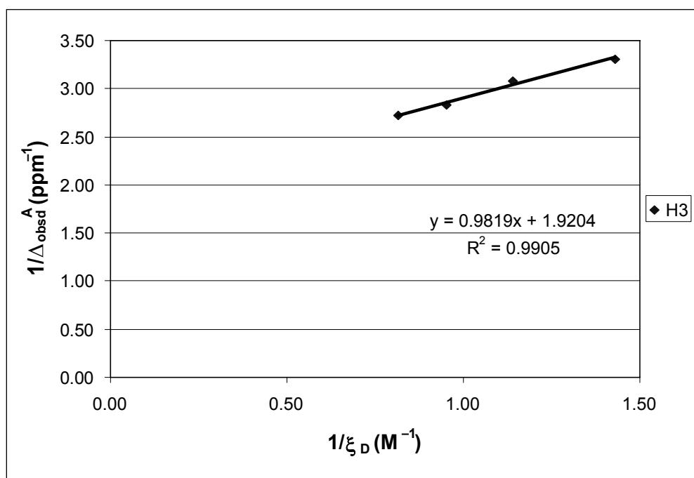
Figure 3 Plot of 1/\Delta_{obs}^A versus 1/\xi_D for the NMR shift of EDNB when complexed with bupivacaine.
