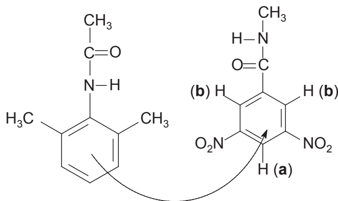
Figure 2 Depiction of electron flow from 2,6-dimethylacetanilide to the aromatic region containing the electron withdrawing nitro groups of 3,5-dinitrobenzamide in the complex of the two.
