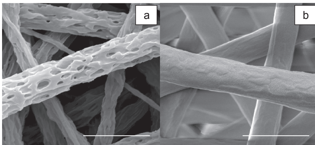
Figure 2 SEM images of 3-D porous fibers (a) after gelatin was leached out of the electrospun Gt/PCL composite fibers (b) (Zhang, Feng et al 2006). Scale bar 2 \mu\text{m} .
