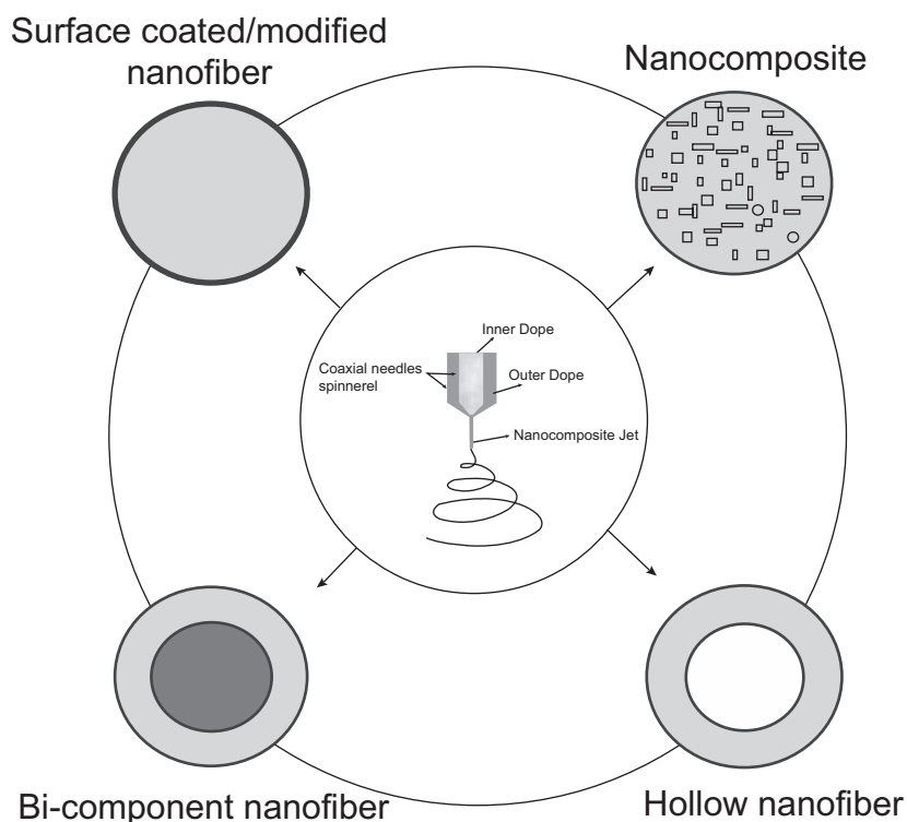
Figure 3 Illustrated cross-sectional views of a variety of novel and functional polymeric nanofibers from coaxial electrospinning, including basic bi-component nanofiber, surface coated/modified nanofiber through tuning the sheath thickness, nanoparticles encapsulated nanocomposite nanofiber, and hollow nanofibers where the core component is removed.
