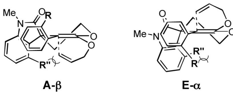
Figure 3. Transition State Models for Claisen Rearrangement of Ketene Acetals 46 and 58
