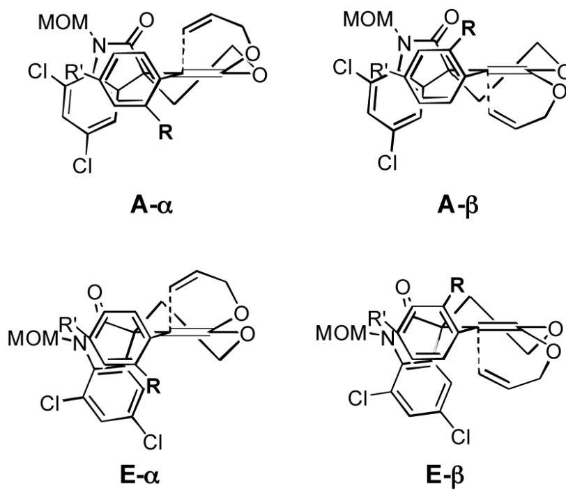
Figure 2. Models for Allylation of Lactones 16 and 29
