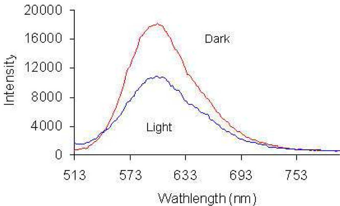
FIGURE 2. Emission spectra of compound 7 ( 5.738 \times 10^{-5} M) in water with excitation at 500 nm.
