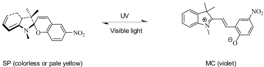
SCHEME 2. Photoisomerization of spiropyran.
