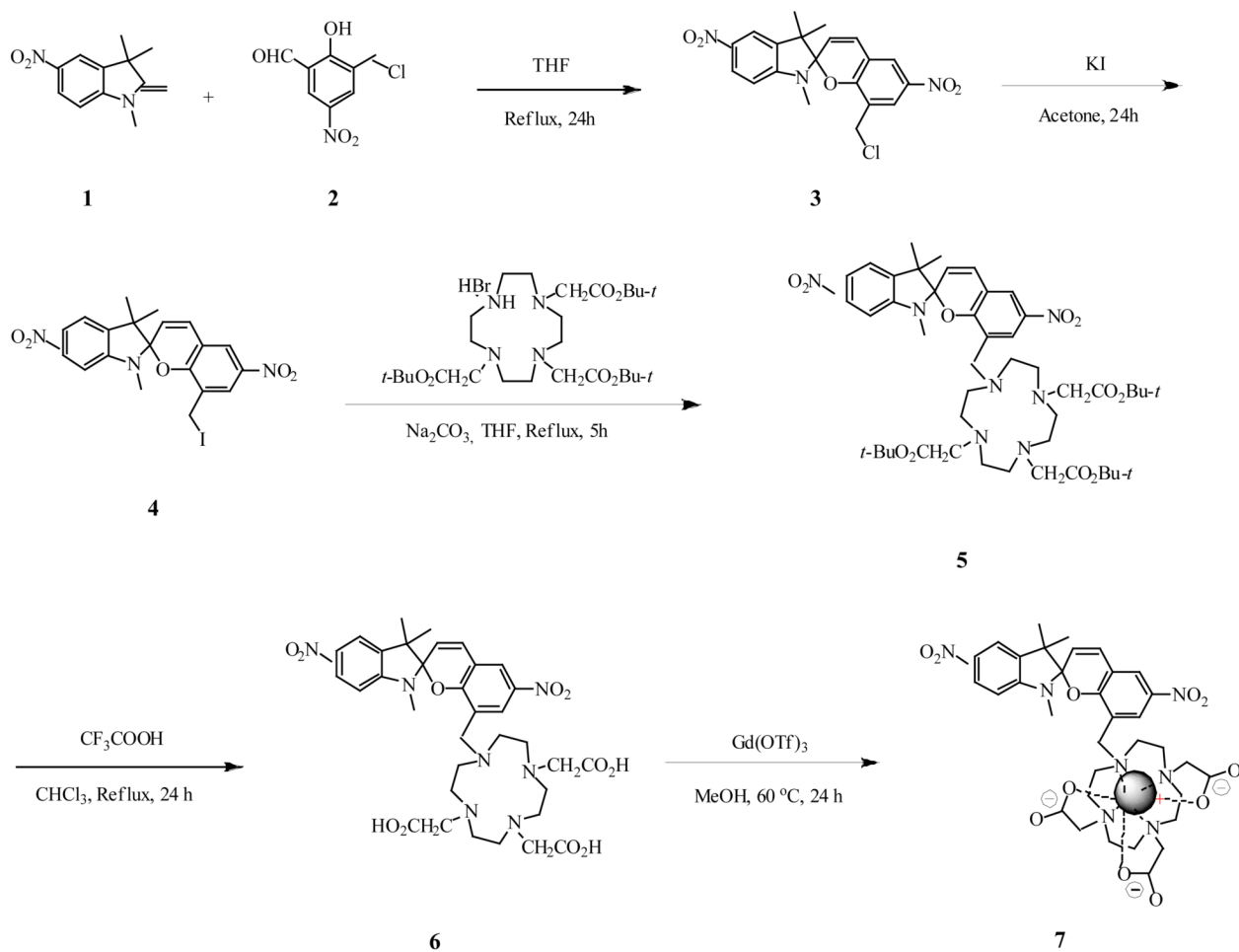
SCHEME 1. Synthesis of dinitrospiropyran-Gd-DO3A complex 7 .
