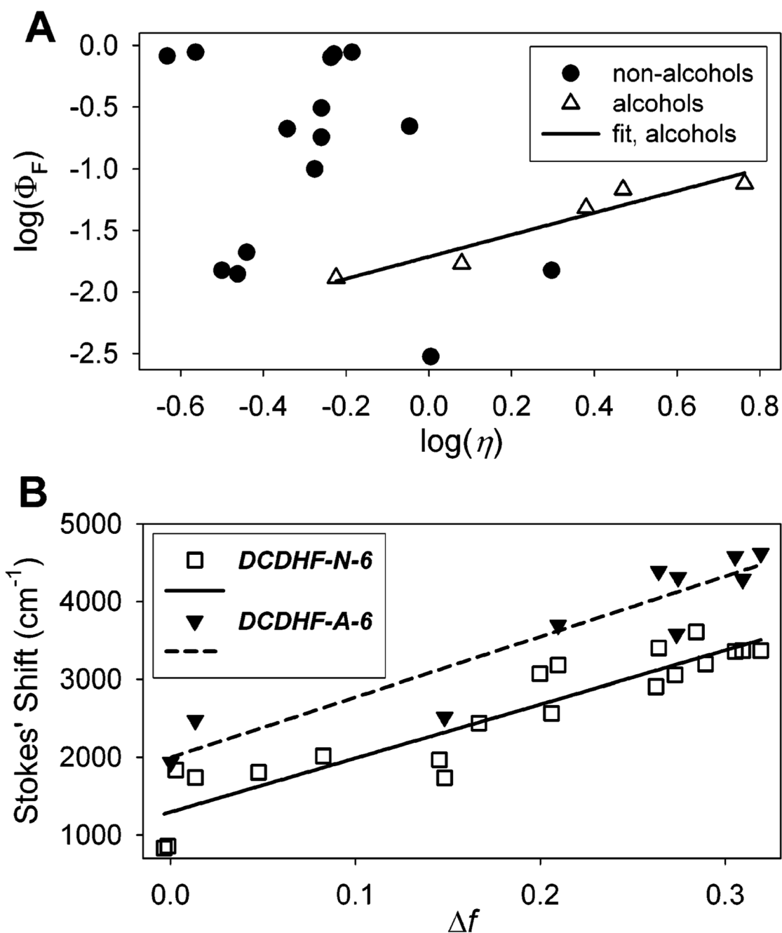
Figure 3. Environment-sensitivity spectroscopic data from Table 2 and Table 3. (A) Log of fluorescence quantum yield as a function of the log of viscosity (relative to water \eta = 1.01 cP) for DCDHF-N-6 . The data for the fluorophore in alcohols are fit by a line with slope of 0.89 ( R^2 = 0.91 ). The fluorophore does not exhibit this obvious trend in other solvents. (B) Lippert plot of emission Stokes shift vs the polarity parameter \Delta f (see text for definition) for DCDHF-N-6 in all solvents in Table 2 and DCDHF-A-6 for a range of solvents. The data for DCDHF-N-6 are fit to a line with slope of 6921 \text{ cm}^{-1} ( R^2 = 0.86 ); the fit for the DCDHF-A-6 data has a slope of 7757 \text{ cm}^{-1} ( R^2 = 0.88 ).
