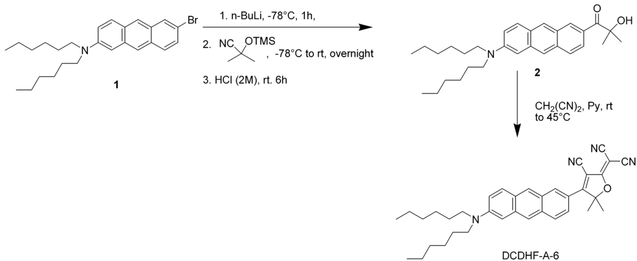
SCHEME 1. Synthesis of DCDHF-A-6
