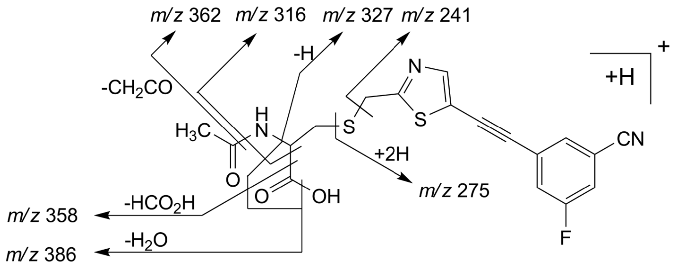
FIG. 8. Proposed fragmentation pathway for ions formed by CID of [M+H]^+ m/z 404 of SP203Nac. The fragmentation accounts for the major ions in the product-ion spectrum of SP203Nac (FIG. 6B)
