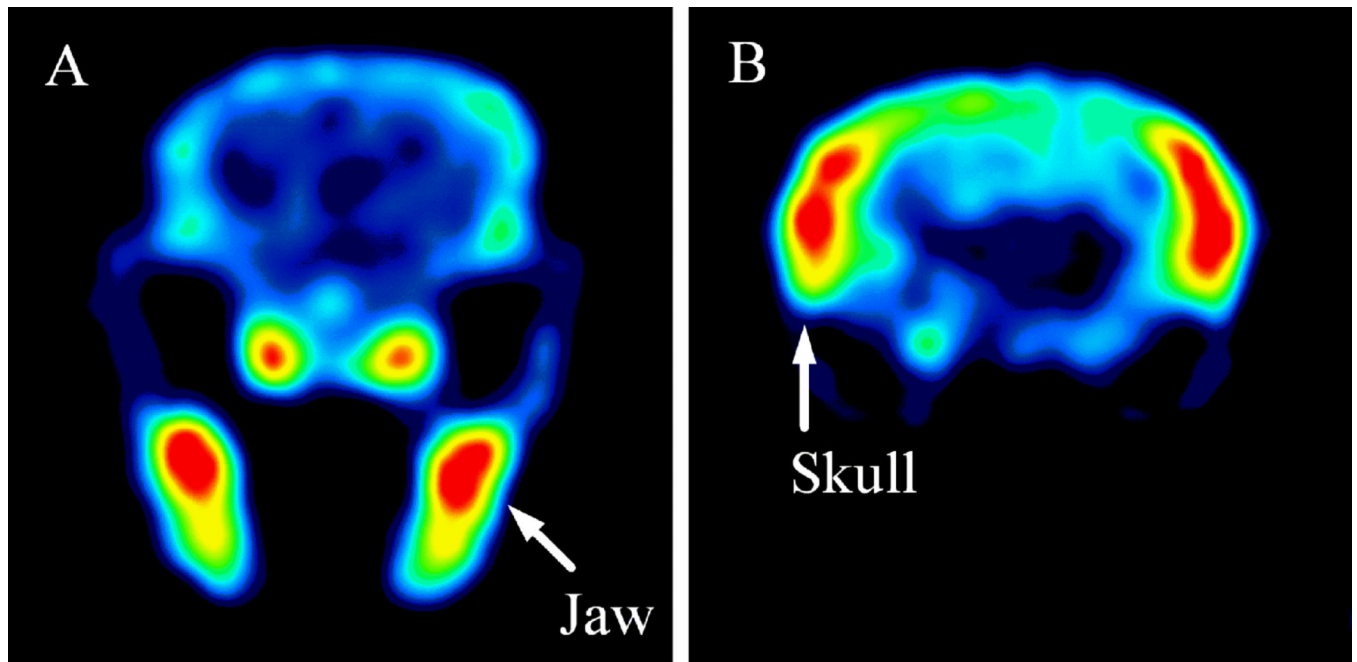
FIG. 4. PET images of a rat head reconstructed from the entire 60 min of emission data after intravenous injection of [ ^{18}\text{F} ]SP203. High radioactivity uptake into the jaw (panel A) and skull (panel B) can be clearly seen.
