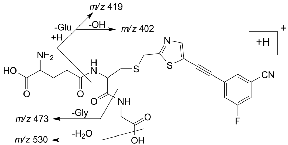
FIG. 7. Proposed fragmentation pathway for ions formed by CID of [M+H]^+ m/z 548 of SP203Glu. The fragmentation accounts for the major ions in the product-ion spectrum of SP203Glu (FIG. 5B)
