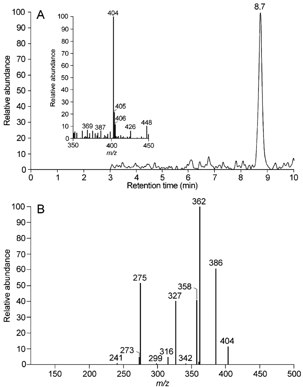
FIG. 6. LC-MS/(MS-MS) analysis of the metabolite SP203Nac in brain extract from rat infused with SP203: mass spectrum (inset) showing [M+H]^+ at m/z 404 and the ion chromatogram for the same ion (A); product-ion spectrum generated by CID of m/z 404 ion (B).
