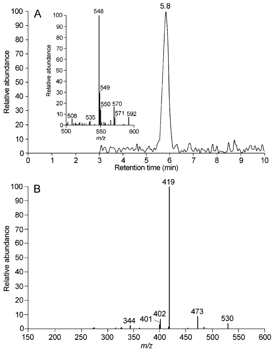
FIG. 5. LC-MS/(MS-MS) analysis of the metabolite SP203Glu in brain extract from rat infused with SP203: mass spectrum (inset) showing [M+H]^+ at m/z 548 and the ion chromatogram for the same ion (A); product-ion spectrum generated by CID of m/z 548 ion (B).
