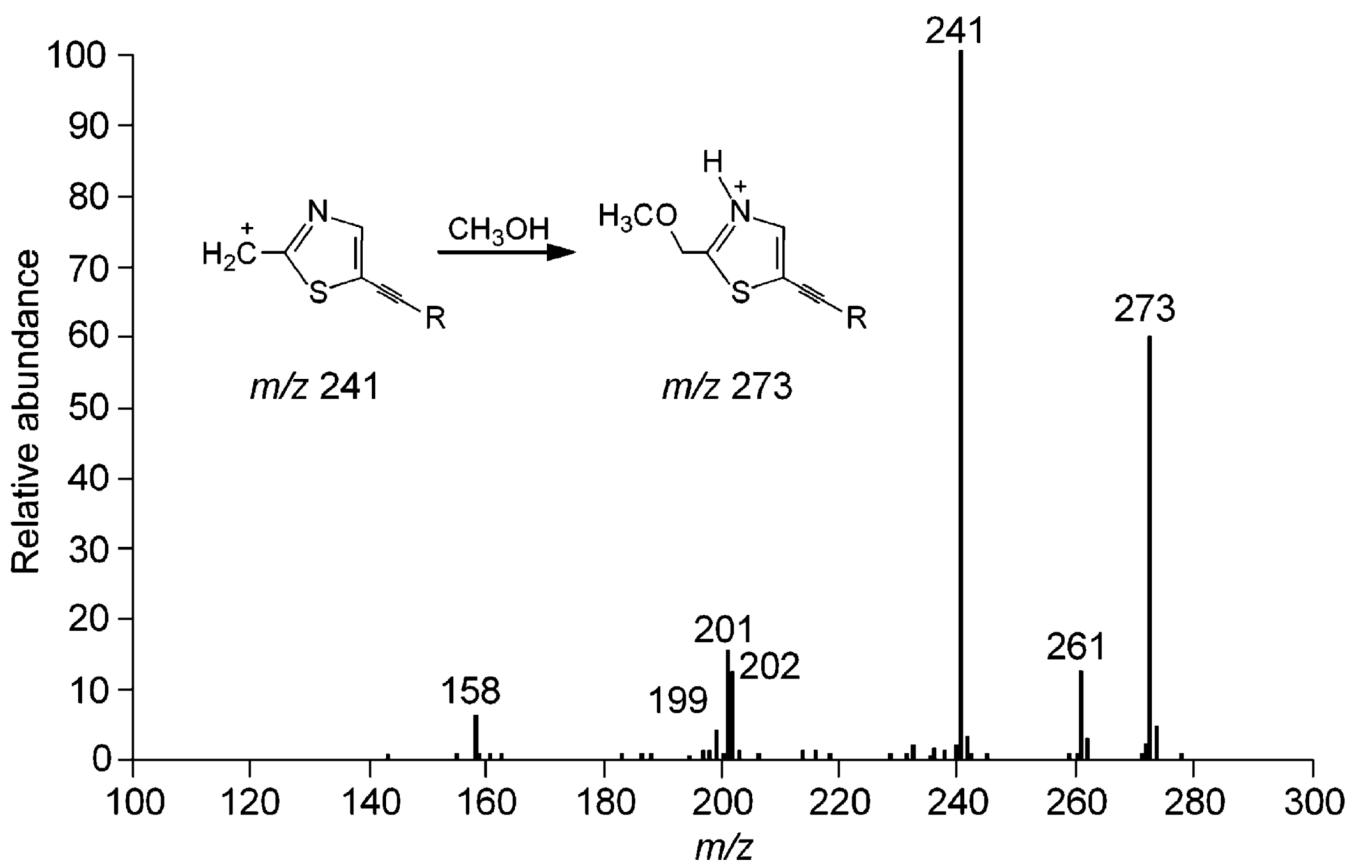
FIG. 9. Product-ion spectrum generated by CID of [M+H]^+ m/z 261 of SP203 and proposed structure (inset) of adduct-ion m/z 273 formed by addition of methanol to m/z 241 ion ( R = 3 -fluoro-5-cyanophenyl). The methanol-adduct formation provided additional proof for the site of glutathione conjugation in SP203Glu
