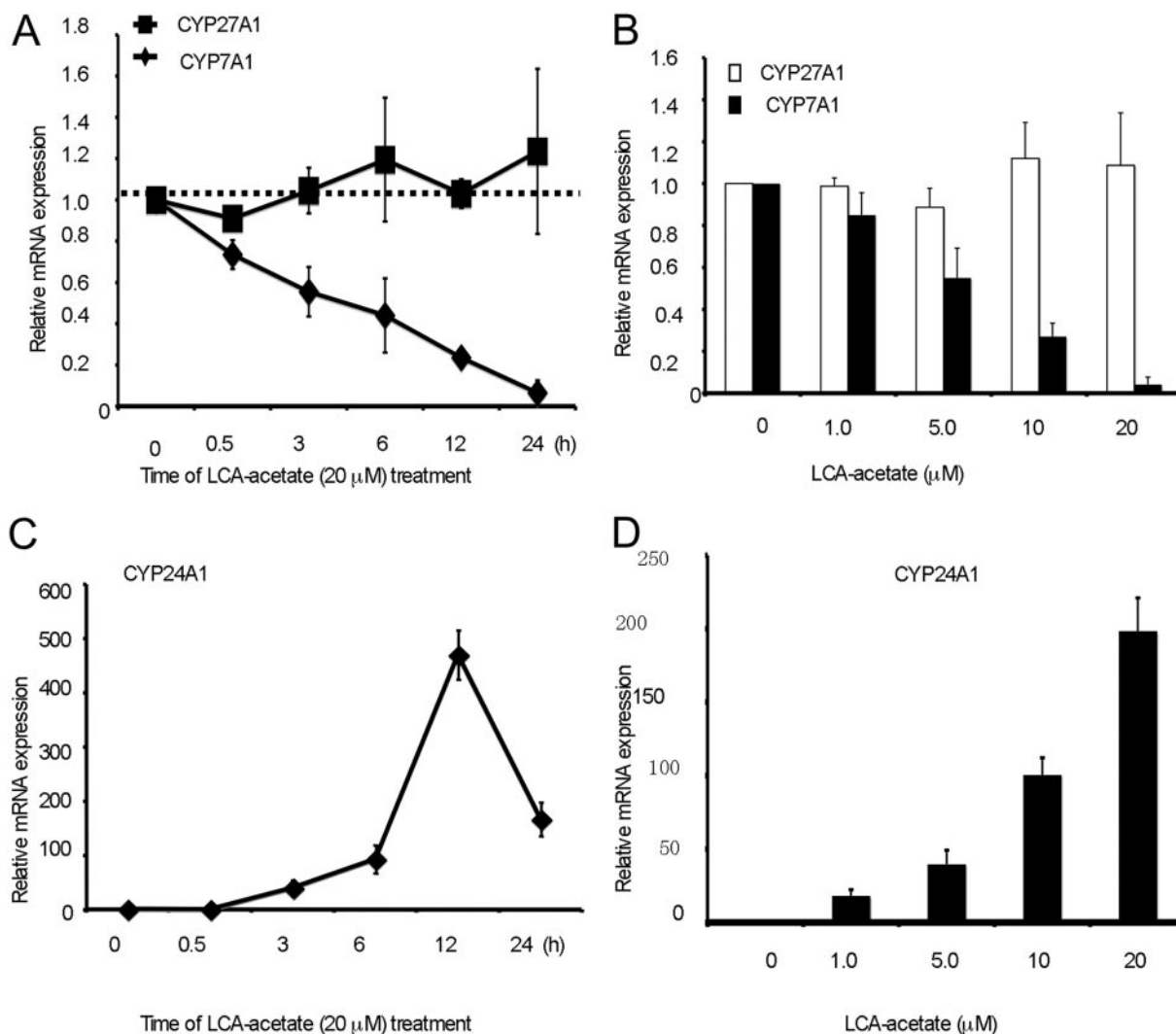
FIG. 2. Real-time PCR assays of the effects of LCA-acetate on CYP7A1 mRNA expression in primary human hepatocytes. Data were pooled from assays using three donor hepatocytes (#HH1403, #HH1410, #HH1412). A, time-dependent effects of LCA-acetate (20 \mu\text{M} ) on CYP7A1 mRNA expression. B, dose-dependent effect of LCA-acetate on CYP7A1 mRNA expression. C, time-dependent effect of LCA-acetate on CYP24A1 mRNA expression. D, dose-dependent induction of CYP24A1 mRNA expression by LCA-acetate. In time course study, primary human hepatocytes were treated with 20 \mu\text{M} LCA-acetate for the time indicated. In dose-dependent study, primary human hepatocytes were treated with increasing doses of LCA-acetate for 24 h. CYP27A1 mRNA expression was assayed as a negative control (A and B). CYP24A1 mRNA expression was assayed as a positive control of VDR induced gene (C and D). Each experiment was done in duplicate, and same experiments were repeated at least five times in each donor hepatocytes.
