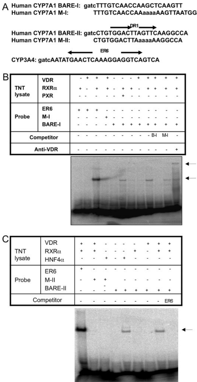
FIG. 5. EMSA of VDR/RXR \alpha binding to human CYP7A1. A, nucleotide sequences of the probes used in the EMSA. Arrows above sequences indicate hormone response element half-sites. Lowercase letters indicate mutations. I, BARE-I; M-I, mutant BARE-I; M-II, mutant BARE-II; DR, direct repeat; ER, everted repeat. B, EMSA of VDR/RXR \alpha binding to human BARE-I probes. VDR/RXR \alpha binding to CYP3A4 ER6 probe and PXR/RXR \alpha binding to BARE-I were used as controls. Excess (50-fold) of unlabeled BARE-I (B-I) and mutant (M-I) probes were used as cold competitor. VDR antibody was used to form a super shift band with VDR/RXR \alpha and BARE-I complex as indicated by an arrow. C, EMSA of VDR/RXR \alpha binding to human BARE II probe. VDR/RXR \alpha binding to CYP3A4 ER6 probe and HNF4 \alpha binding to BARE-II were used as controls. Excess (50-fold) of unlabeled ER6 probes were used as cold competitor. Each EMSA binding reaction contained 2 \mu l of \alpha - 32 P-labeled probes ( 2 \times 10^4 cpm) incubated with in vitro-synthesized proteins (TNT lysate) for 20 min before loaded into the gel.
