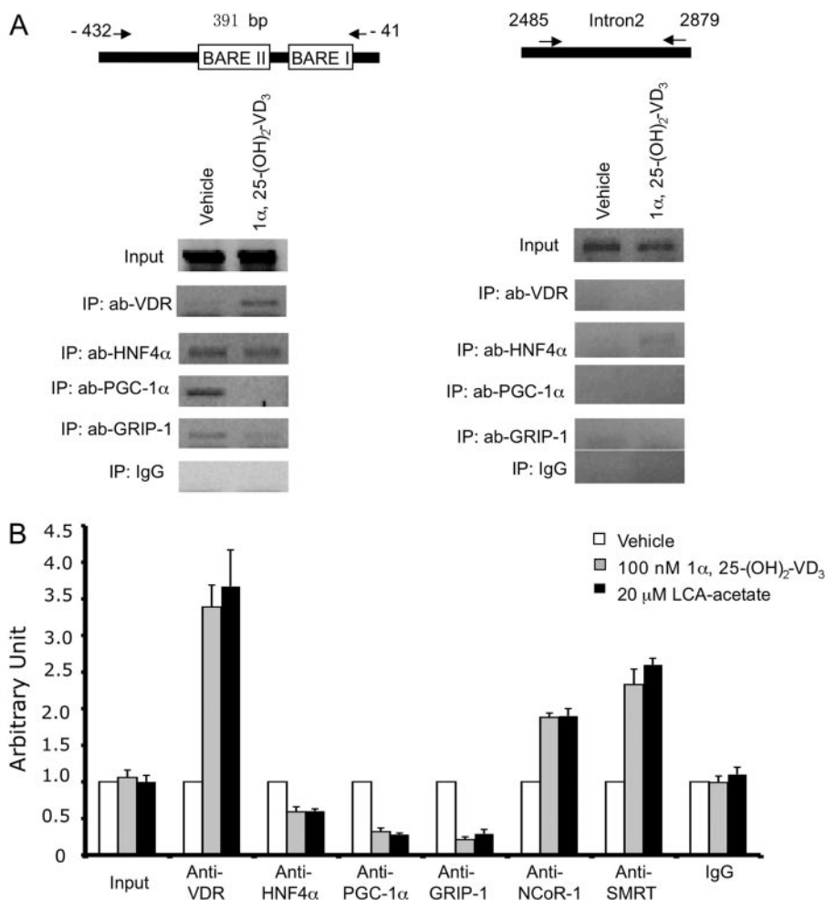
FIG. 8. ChIP assay of the effect of 1 \alpha , 25-(OH) _2 -VD _3 on CYP7A1 chromatin structure in primary human hepatocytes and HepG2. A, ChIP assay of CYP7A1 chromatin containing the BARE-I and BARE-II (nt -432 to -41). Primary human hepatocytes (HH1432) were treated with vehicle (EtOH) or 1 \alpha , 25-(OH) _2 -VD _3 (100 nM) for 16 h. An antibody against VDR, HNF4 \alpha , PGC-1 \alpha , GRIP-1, or nonimmune IgG (IgG, as a negative control) was used to precipitate chromatin fragments. Five-percent cell extracts were set aside as input. PCR primers were used to amplify the region from -432 to -41 of CYP7A1 promoter, and the intron 2 region of CYP7A1 from nt 2485 to 2879 as a negative control. B, Q-PCR assay of CYP7A1 chromatin containing the BARE-II (nt -180 to -111, the HNF4 \alpha binding site) HepG2 cells were treated with vehicle (EtOH), 1 \alpha , 25-(OH) _2 -VD _3 (100 nM), or LCA-acetate (20 \mu M) for 24 h. An antibody against VDR, HNF4 \alpha , PGC-1 \alpha , or GRIP-1, NCoR-1, SMRT, or nonimmune IgG was used to precipitate chromatin fragments. TaqMan primers/probe sets were used for Q-PCR assay of the amount of transcription factor binding to the CYP7A1 chromatin containing the HNF4 \alpha binding site (nt -180 to -111) as described under Materials and Methods .
