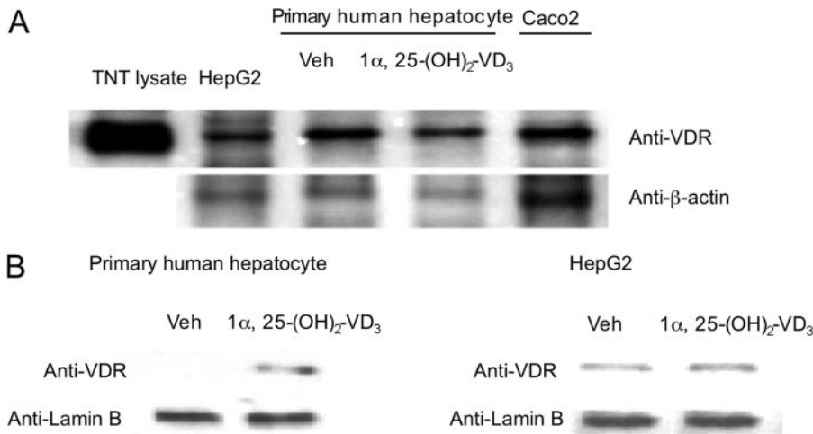
FIG. 1. Immunoblot analysis of the VDR protein expression and cellular distribution in HepG2 and primary human hepatocytes. A, immunoblot of VDR protein expression in total cell lysates of HepG2 and primary human hepatocytes (#HH1320). In vitro-synthesized human VDR protein was loaded as the molecular marker. Human primary hepatocytes were treated with vehicle (EtOH) or 1\alpha, 25-(OH)_2-VD_3 (50 nM) for 6 h. \beta -Actin protein expression was monitored as the internal loading control. B, immunoblot of VDR in the nuclear fractions of primary human hepatocytes (#HH1391) and HepG2. Cells were treated with vehicle (EtOH) or 50 nM 1\alpha, 25-(OH)_2-VD_3 for 6 h. Lamin B protein levels in nuclei were monitored as the internal loading control.
