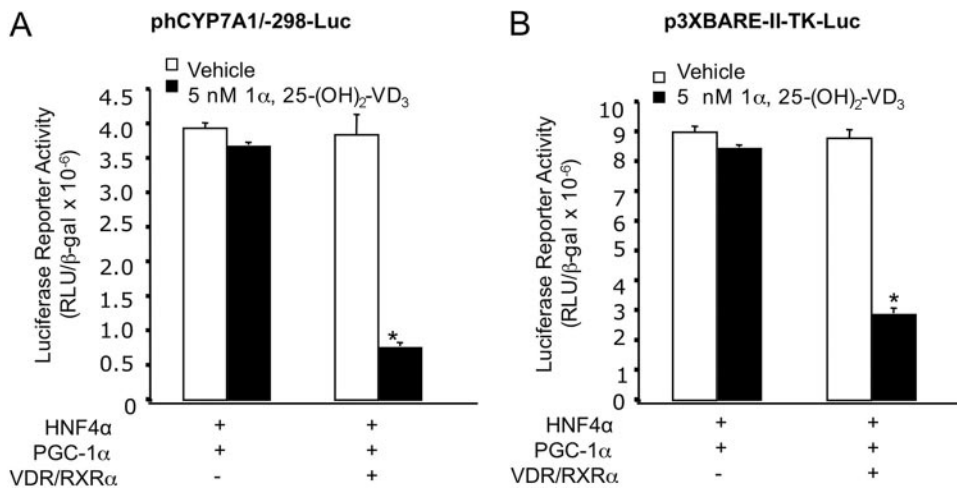
FIG. 6. Reporter assays of the effects of VDR on CYP7A1 gene transcription in HepG2 cells. A, the human CYP7A1 promoter luciferase reporter pHCYP7A1/298-Luc was used to assay the effect of HNF4 \alpha , PGC-1 \alpha , and VDR/RXR \alpha on reporter activity with or without 1\alpha, 25-(OH)_2-VD_3 . B, reporter assay of a heterologous reporter (p3XBARE II-TK-Luc) containing three copies of the BARE-II sequence of human CYP7A1 linked to TK-Luc promoter. After transfecting for 24 h, cells were treated with EtOH or 5 nM 1\alpha, 25-(OH)_2-VD_3 for 16 h before harvesting. The luciferase activity was normalized by \beta -galactosidase activity. Each experiment was done in duplicate, and the same experiment was repeated four times. An * indicated statistically significant difference, p < 0.05 , 1\alpha, 25-(OH)_2-VD_3 -treated versus control.
