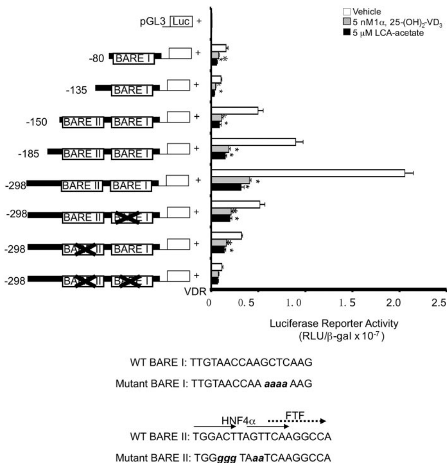
FIG. 4. Reporter assays of the effects of 1\alpha, 25\text{-(OH)}_2\text{-VD}_3 and LCA-acetate on CYP7A1 luciferase reporter activities. CYP7A1 promoter deletion reporter constructs (0.2 \mu\text{g} ) or empty reporter vector pGL3-basic was cotransfected with VDR (0.1 \mu\text{g} ) into HepG2 cells. CYP7A1 wild-type promoter reporter construct phCYP7A1/–298, reporter with mBARE-I, mBARE-II, or the BARE-I and -II double mutation (mBARE-I and -II) (0.2 \mu\text{g} ) was cotransfected with VDR expression plasmid (0.1 \mu\text{g} ) into HepG2 cells. The mutant sequences are shown. After transfecting for 24 h, cells were treated with vehicle (EtOH), 1\alpha, 25\text{-(OH)}_2\text{-VD}_3 (5 nM), or LCA-acetate (5 \mu\text{M} ) for 16 h before harvesting. The luciferase activity was normalized by \beta -galactosidase activity. Each experiment was done in duplicate, and the same experiment was repeated five times. An * indicates statistically significant difference, p < 0.05 , 1\alpha, 25\text{-(OH)}_2\text{-VD}_3 - or LCA-acetate-treated versus vehicle control.
