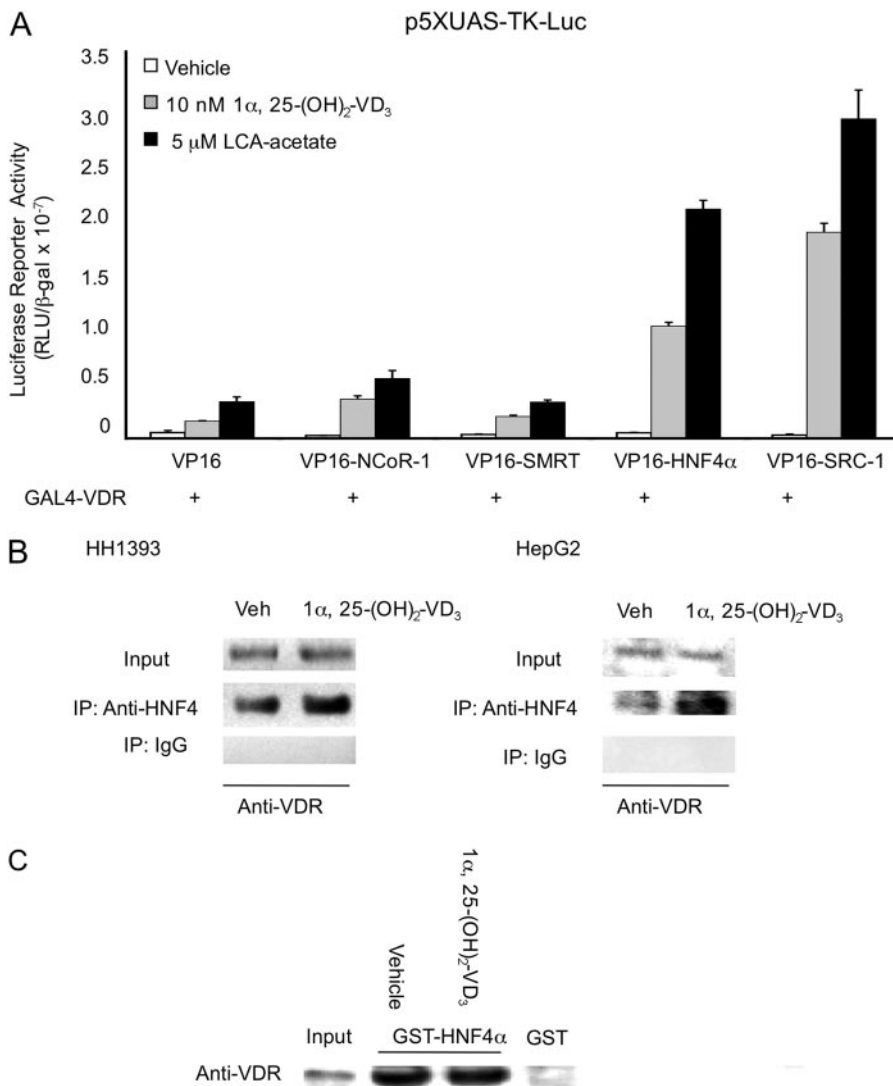
FIG. 7. VDR interacts with HNF4 \alpha . A, mammalian two-hybrid assay of VDR and HNF4 \alpha interaction. The reporter construct p5XUAS-TK-Luc (0.2 \mu g) was transfected into HEK293 cells, and 0.1 \mu g of GAL4-VDR was cotransfected with 0.1 \mu g of VP16 empty vector, VP16-SRC-1, VP16-NCOR-1, VP16-SMRT, or VP16-HNF4 \alpha into HEK293 cells. After 24 h, cells were treated with vehicle (EtOH), 1\alpha, 25-(OH)_2-VD_3 (10 nM), or LCA-acetate (5 \mu M) for 16 h before harvesting. The experiment was done in duplicate, and the same experiment was repeated four times. An * indicates statistically significant difference, p < 0.05 1\alpha, 25-(OH)_2-VD_3 - or LCA-acetate-treated versus control. B, CoIP assay of HNF4 \alpha and VDR interaction. Primary human hepatocytes (HH1393) and HepG2 cells were treated with vehicle (EtOH) or 1\alpha, 25-(OH)_2-VD_3 (100 nM) for 6 h. Whole cell extracts were incubated with an HNF4 \alpha antibody or nonimmune IgG. Coprecipitated VDR was detected by a VDR antibody. C, bacterium protein extracts containing GST-HNF4 \alpha or GST were immobilized to glutathione beads for 16 h at 4°C. GST-HNF4 \alpha -bound beads were incubated with 1 mg of protein extracts isolated from HepG2 cells treated with vehicle (EtOH) or 1\alpha, 25-(OH)_2-VD_3 (100 nM) for 24 h at 4°C. VDR protein was detected by immunoblotting. Thirty-five micrograms of HepG2 protein extract was loaded as input.
