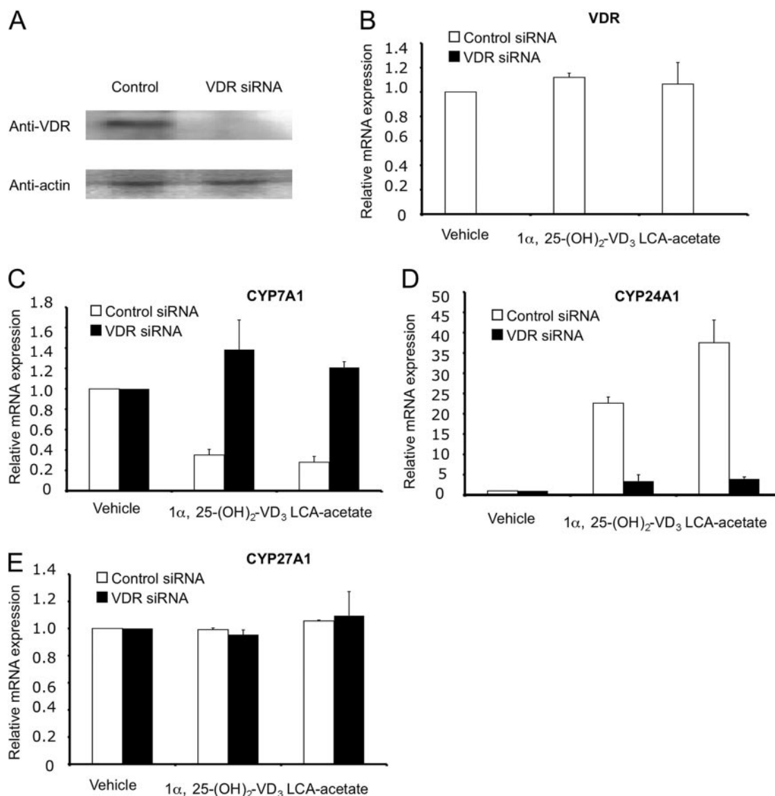
FIG. 3. The siRNA knockdown of VDR prevents ligand-dependent VDR inhibition of CYP7A1 expression in HepG2 cells. HepG2 cells were transfected with the SMARTpool siRNA to VDR or control siRNA and incubated for 72 h. Cells were then treated with vehicle (EtOH), 1 \alpha , 25-(OH) _2 -VD _3 (100 nM), or LCA-acetate (20 \mu M) for 24 h. Cells extracts were isolated for immunoblot analysis of VDR protein expression (A). Total RNA was isolated for real-time PCR analysis of VDR (B), CYP7A1 (C), CYP24A1 (D), CYP27A1 (E) mRNA levels. Data show relative mRNA expression of VDR siRNA treated to the control siRNA-treated samples. Data represent the mean \pm S.D. of at least three individual experiments.
