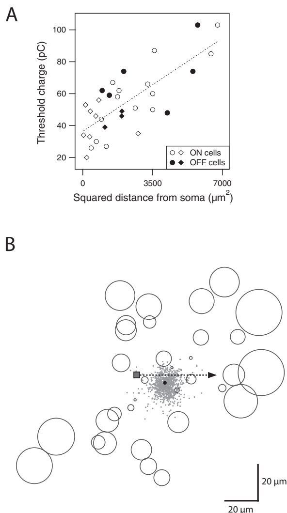
Figure 4. Sensitivity to spatial location of stimulation. A , Threshold charge plotted against the square of the distance between stimulation electrode and estimated soma location. Most data are from stimulating at a neighboring electrode (circles), but several cells stimulated directly at the primary electrode were included (diamonds). The dashed line is a linear fit to the data ( R^2 = 0.58 ) and denotes a squared dependence of charge on distance from soma. B , Stimulation sites (circles) plotted relative to the soma center (filled square). Data from all cells were aligned at the soma center and rotated so that the direction of the axon (dotted arrow) points to the right. Circle diameter is proportional to the threshold charge minus an offset (minimum 26 pC, maximum 103 pC). The lowest thresholds are found near the soma and the proximal portion of the axon. The filled circle indicates the center of a Gaussian fit to the data and the gray dots denote the expected error around this center (resampled 950 times with replacement; see Materials and Methods). This location of maximal sensitivity to electrical stimulation is situated \sim 13 \mu\text{m} to the right of the soma center.
