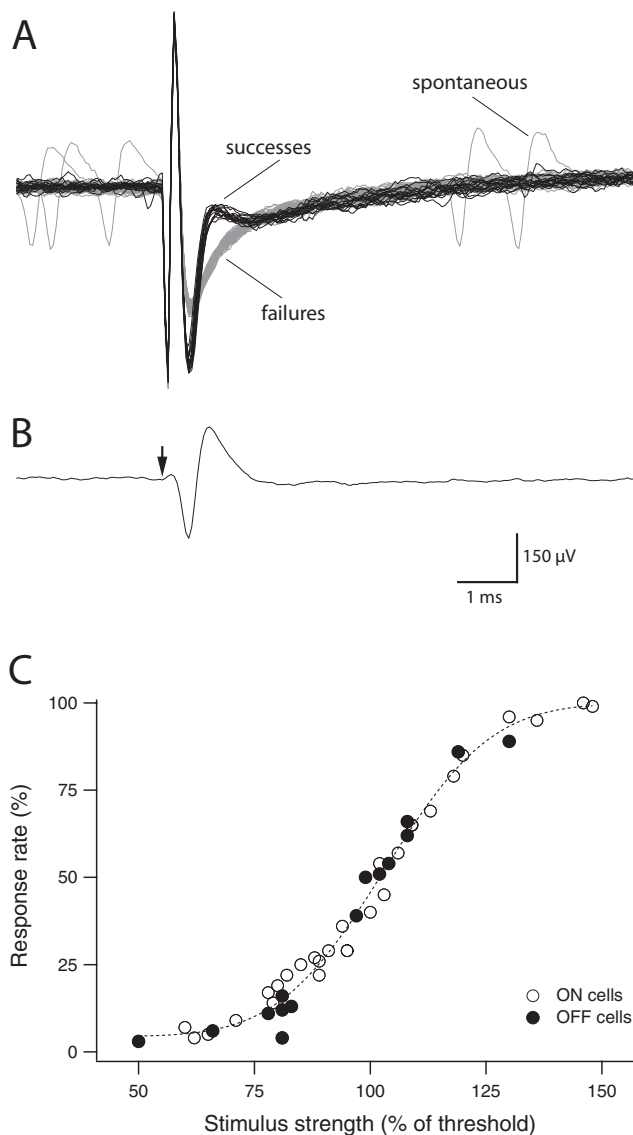
Figure 2. Spike responses to electrical stimulation. A , Spikes recorded in the same ON cell shown in Figure 1A, stimulated using a neighboring electrode. A superposition of responses to 65 repeated pulses of 50 \mu s duration is shown. Near threshold, the electrical stimulus (large artifact) evoked either successful spikes (black traces) or no spikes (gray traces). Occasional spontaneous spikes also occurred before and after the stimulation. B , The average evoked spike, obtained by subtracting failures from successes in A . The evoked spike resembles the spontaneous spikes in A . The arrow points to the onset of the stimulation pulse. C , Response rate (fraction of pulses that evoked a spike) as a function of stimulus strength. Threshold was defined as a 50% response rate. Data from 18 parasol cells were pooled for this plot; open and closed symbols denote ON and OFF cells, respectively. The dashed line is an error function fit to the data (see Materials and Methods).
