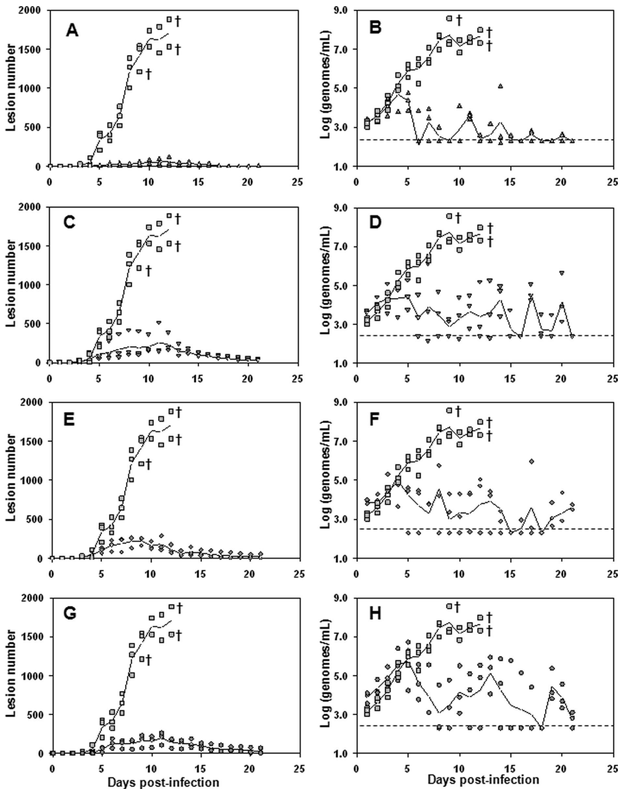
FIG. 2. Average lesion number and viral load of NHP (three NHP per treatment group) infected with 5 \times 10^7 PFU of MPX and treated with either vehicle alone or ST-246 administered once per day for 14 days starting at day 3 postinfection. Viral lesion numbers (A, C, E, and G) and DNA levels (B, D, F, and H) were measured for animals treated with vehicle (squares) or ST-246 at 100 mg/kg (A and B; triangles), 30 mg/kg (C and D; inverted triangles), 10 mg/kg (E and F; diamonds), or 3 mg/kg (G and H; circles). Each symbol represents the data for an individual animal. The data from the vehicle-treated animals is included in each panel for comparison purposes. The geometric mean is shown as a solid line through the data points. The lower limit of quantification for DNA levels measured by quantitative PCR assay is shown as a black dashed line. All vehicle-treated animals either died or were euthanized (daggers) due to MPX infection between day 11 and 14 postinfection. A one-way ANOVA model generated a P value of <0.001 for all treatment groups compared to the results for the vehicle-treated control group.
