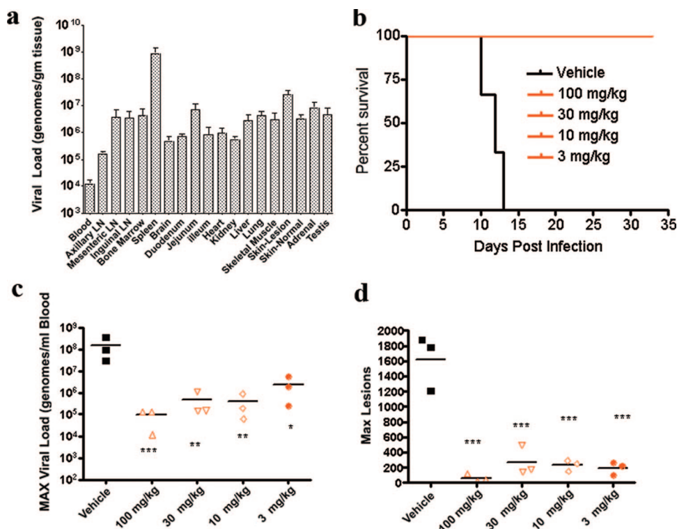
FIG. 1. Disease outcomes for NHP (three NHP per treatment group) infected with 5 \times 10^7 PFU of MPX and treated with either vehicle alone or ST-246 administered at 3, 10, 30, or 100 mg/kg/day starting at day 3 postinfection. (a) Virus level in tissues 3 dpi and just prior to initiation of drug treatment. (b) Kaplan-Meier survival curve (log-rank test, all ST-246 groups, P < 0.001 ). (c) Maximum viral DNA by treatment and day postinfection. Bars, means; triangle, individual values (for 100-mg/kg ST-246-treated group, P < 0.001 ; for 30- and 10-mg/kg ST-246-treated groups, P < 0.01 ; for 10-mg/kg ST-246-treated group, P < 0.05 ). (d) Maximum lesion count by treatment group. Bars, means; triangles, individual values (for all ST-246-treated groups, P < 0.001 ).
