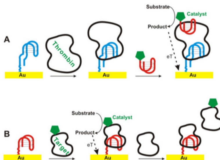
Figure 32. (A) Sandwich assays for electrochemical thrombin detection. (B) Competitive assays based on electrochemical aptamer sensors.
