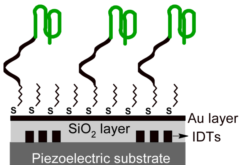
Figure 37. A scheme of an aptamer sensor based on the change in surface acoustic waves. The aptamer is shown in green, which is attached to the gold surface via a DNA spacer (in black). 524
