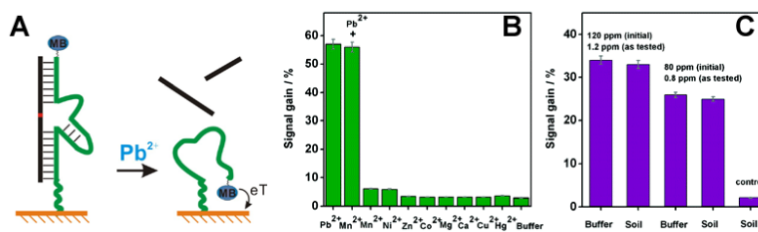
Figure 12. Electrochemical Pb 2+ detection. (A) Schematics of the sensor design. (B) Metal-dependent sensor response. (C) Detection of Pb 2+ in soil samples. Reprinted with permission from Reference 283. Copyright 2007 American Chemical Society.
