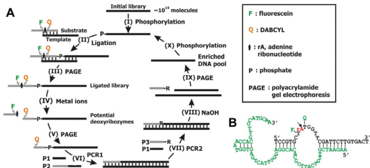
Figure 8. (A) Schematic of in vitro selection of signaling DNazymes. See text for descriptions. (B) Secondary structure of the DET22-18 DNzyme. F and Q are fluorescein and Dabcyl, respectively. Reprinted with permission from Reference 158. Copyright 2003 American Chemical Society.
