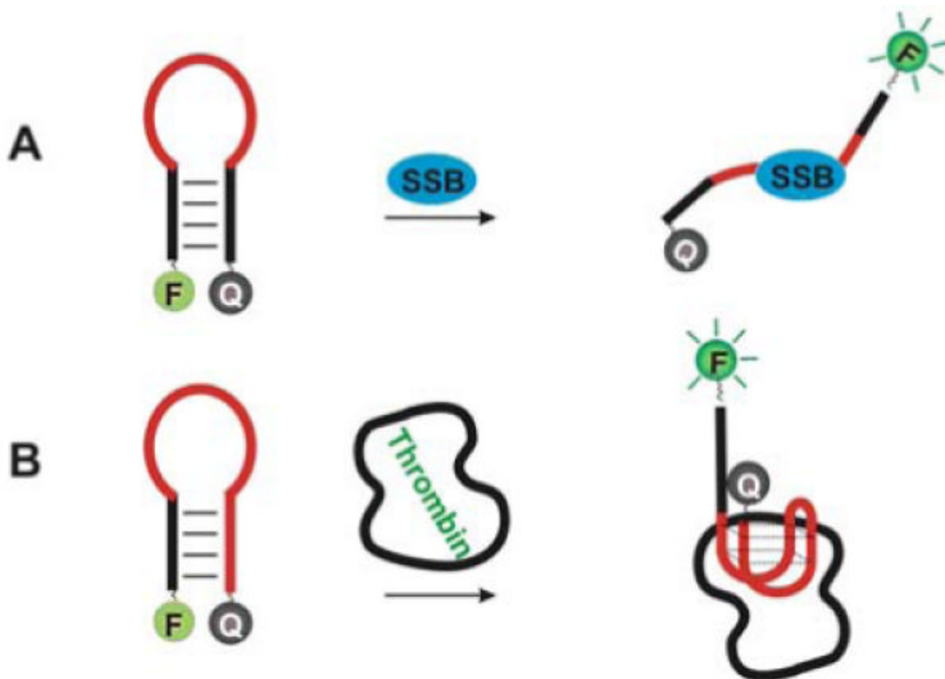
Figure 20. Aptamer beacons. (A) Application of molecular beacons to probe single-stranded DNA binding proteins (SSB). 363 (B) Detection of thrombin with an aptamer beacon. The aptamer contained an extension (in black), which formed the stem part of the hairpin. Binding to thrombin opened the hairpin and increased fluorescence. 364
