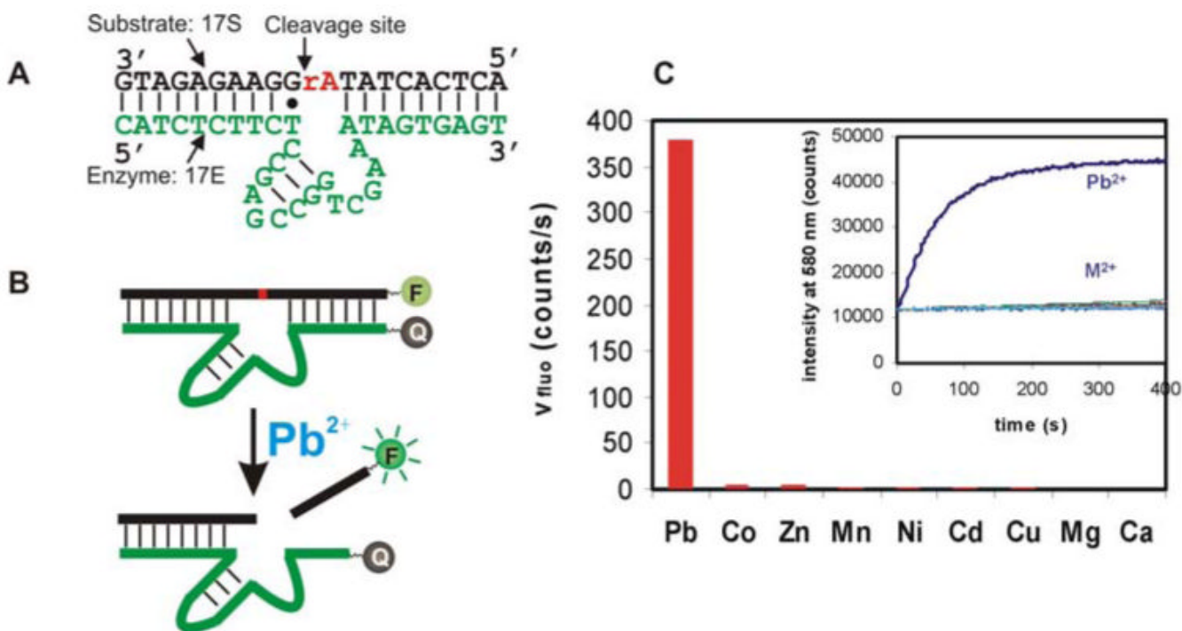
Figure 4. A catalytic beacon \text{Pb}^{2+} sensor. (A) The secondary structure of the \text{Pb}^{2+} -specific DNAzyme. (B) Schematics of beacon signal generation. (C) Selectivity of the sensor. Inset: Kinetics of fluorescence increase with \text{Pb}^{2+} and other divalent metal ions. Reprinted with permission from Reference 186. Copyright 2006 American Chemical Society.
