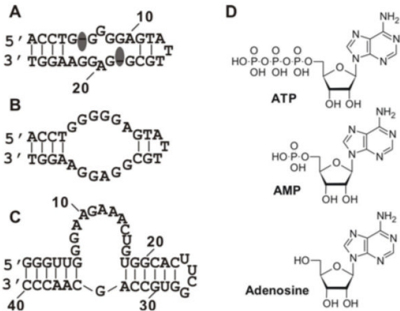
Figure 15. (A) The ATP-binding DNA aptamer with bound ATP. 30 (B) An alternative way of drawing the aptamer in (A). (C) The ATP binding RNA aptamer. 313 (D) Structure of ATP, AMP, and adenosine.
