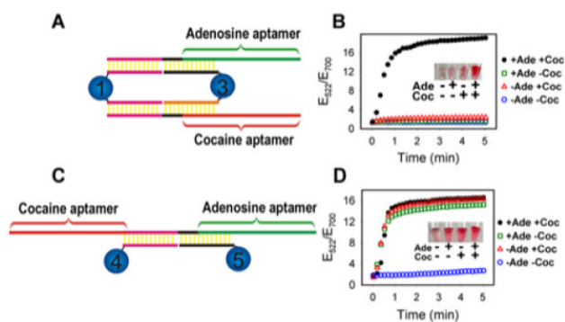
Figure 28. Colorimetric sensors that change color only when both adenosine and cocaine are present (A) or either analyte is present (C). Kinetics ((B) and (D)) of color change of the aggregates in the presence of 1 mM adenosine, 1 mM cocaine, 0.5 mM adenosine and 0.5 mM cocaine, or no analytes in (A) and (C), respectively. Insets show the colors displayed by the sensors. Reprinted with permission from Reference 448. Copyright 2006 John Wiley & Sons, Inc.
