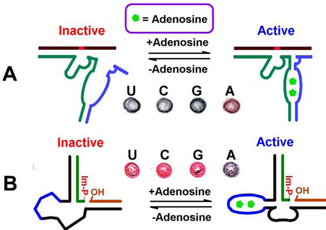
Figure 44. Colorimetric aptazyme sensors for adenosine based on RNA-cleaving enzymes (A) and DNA ligation enzymes (B). Reprinted with permission from Reference 197. Copyright 2004 American Chemical Society.
