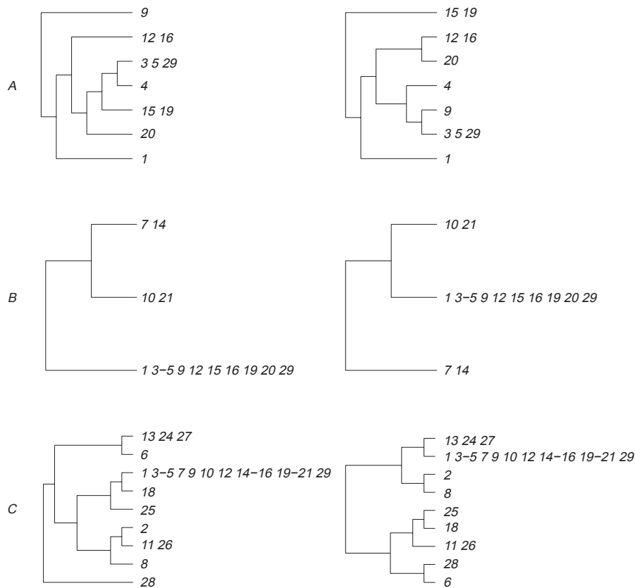
Figure 7. The three pairs of clusters A, B, and C corresponding to Figure 6 for which HYBRIDNUMBER (separately) calculates the minimum number of hybridization events (left: ITS , right: phyB ).
