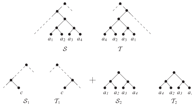
Figure 4. Two rooted binary phylogenetic trees S and T divided under the cluster reduction rule. The hybridization number of S and T is the sum of the hybridization numbers of S_1 and T_1 , and S_2 and T_2 .
