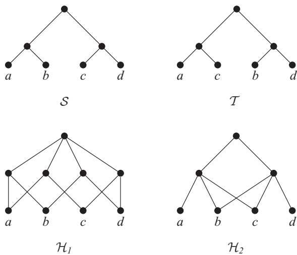
Figure 1. Two rooted binary phylogenetic trees S and T and the two hybridization networks \mathcal{H}_1 and \mathcal{H}_2 which explain both trees.
