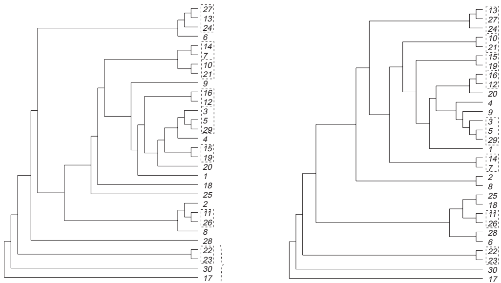
Figure 5. The input to HYBRIDNUMBER for the combination phyB and ITS . Restricting to overlapping taxa, the tree resulting from the nuclear sequence ITS is on the left, while the tree resulting from the chloroplast sequence phyB is on the right. Labels in boxes denote the eight maximal pendant subtrees that are common to both trees, and the brace denotes a maximal chain once we have applied the subtree reductions.
