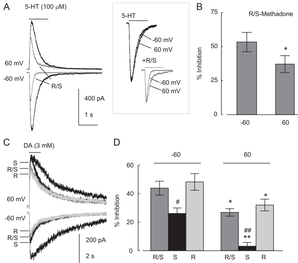
Fig. 7. Voltage-dependent inhibition by methadone of 5-HT 3AB receptors is independent of desensitization. A , 5-HT 3AB receptor-mediated currents evoked by 5-HT (100 μM) applied for 1 s either alone (in black) or simultaneously with ( R/S )-methadone (100 μM; in gray) at holding potentials of -60 and 60 mV. Inset, currents recorded at -60 and 60 were normalized and superimposed to compare kinetics. The time course of desensitization of 5-HT-evoked currents recorded at both potentials in the absence of ( R/S )-methadone (black traces) was similar. In the presence of ( R/S )-methadone (gray traces), 5-HT-evoked currents decayed faster at -60 mV. B , percentage of inhibition at -60 and 60 mV ( n = 5 ). The inhibition by ( R/S )-methadone was significantly smaller at 60 mV than at -60 mV (*, p < 0.05 ; paired t test). Vertical lines are \pm S.E.M. C , 5-HT 3AB receptor-mediated currents evoked by dopamine (DA; 3 mM) applied for 1 s either alone (in black) or simultaneously with 100 μM ( R/S )- (medium gray), ( R )- (light gray), or ( S )- (dark gray) methadone at holding potentials of -60 and 60 mV. D , percentage of inhibition at -60 and 60 mV ( n = 5 ). The inhibitions by all three methadone formulations were significantly smaller at 60 mV than at -60 mV (*, p < 0.05 ; **, p < 0.01 ; paired t test). Furthermore, inhibition by ( S )-methadone was significantly smaller than ( R )-methadone at -60 mV (#, p < 0.05 ) and both ( R/S )- and ( R )-methadone at 60 mV (##, p < 0.001 ) as determined by ANOVA with post hoc Dunnett's test. Vertical lines are \pm S.E.M.
