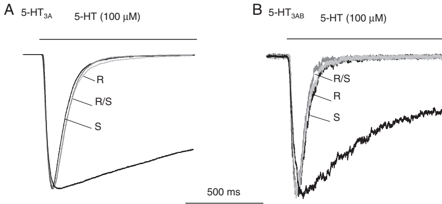
Fig. 4. ( R )- and ( S )-Methadone increase 5-HT 3 receptor apparent desensitization. Superimposed and normalized 5-HT (100 \mu M)-evoked currents recorded from cells expressing either 5-HT 3A (A) or 5-HT 3AB (B) receptors. In each case, currents were recorded from the same HEK cell in the absence and presence of ( R/S )-, ( R )-, or ( S )-methadone (100 \mu M).
