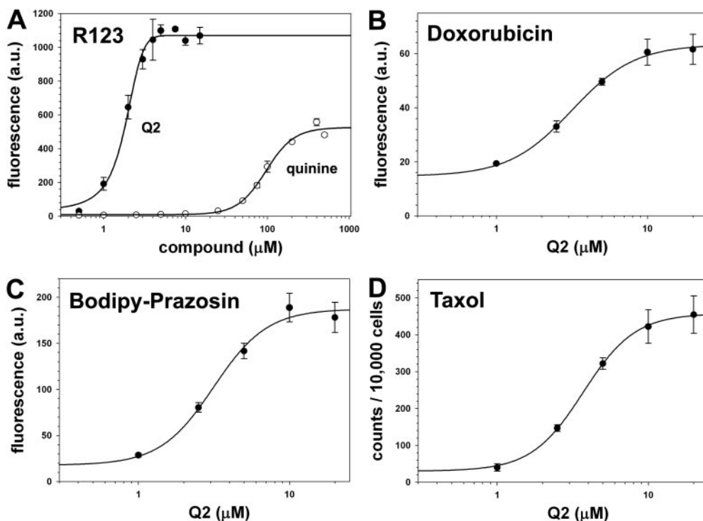
Fig. 2. Concentration-dependent inhibitory potency of Q2 on the transport of different P-gp substrates using MCF-7/DX1 cells. A–C, MCF-7/DX1 cells were treated with R123 ( 1.3 \mu\text{M} ), doxorubicin ( 3 \mu\text{M} ), or BODIPY-FL-prazosin ( 0.5 \mu\text{M} ) and various concentrations of inhibitors for 30 min at 37^\circ\text{C} as described under Materials and Methods . Cells were analyzed for fluorescence using a FACSCalibur flow cytometer. D, MCF-7/DX1 cells were treated with [ ^3\text{H} ]paclitaxel ( 7.5 \text{ nM} ) and various concentrations of Q2 for 40 min at 37^\circ\text{C} , then with trypsin for 1 h at 37^\circ\text{C} . Cells were analyzed for accumulation of the radioactive paclitaxel using a scintillation counter.
