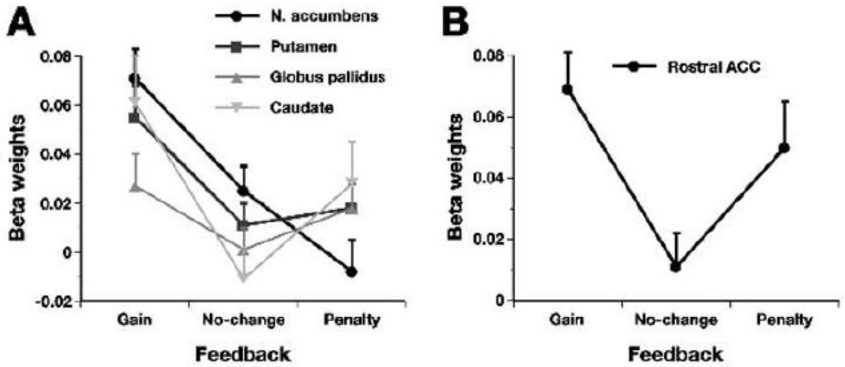
Figure 2. Mean beta weights (and standard errors) in (A) the four basal ganglia regions and (B) the rACC in response to monetary gains, no-change feedback, and monetary penalties (averaged across hemispheres). Note that only the nucleus accumbens (NAcc) showed a trend for smaller responses to penalties relative to no-change feedback.
