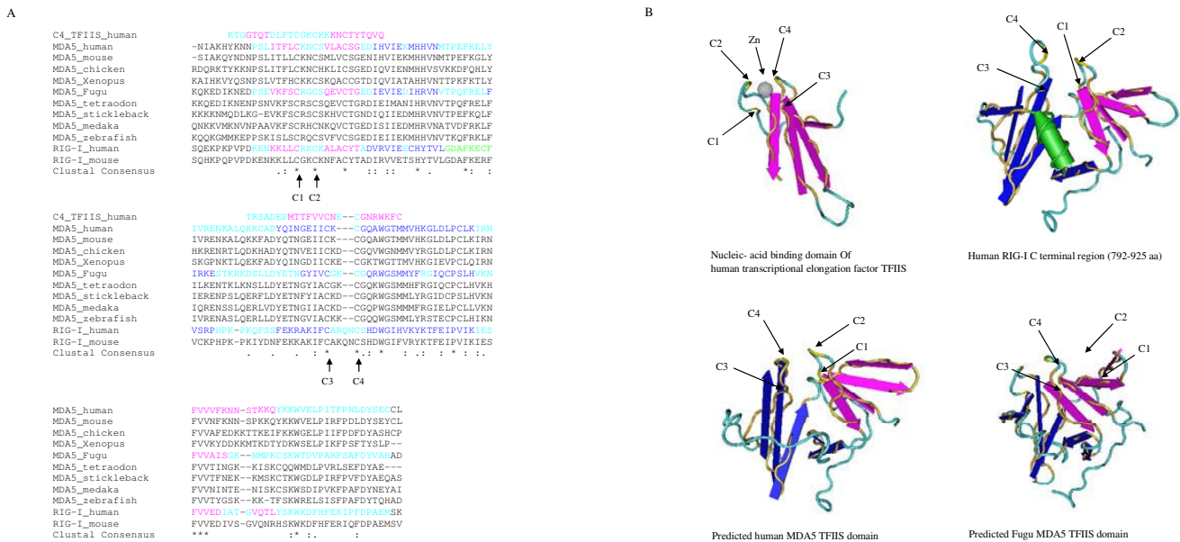
Figure 6 Multiple alignment (A) and structural modelling (B) of TFIS domains. The domain sequences were predicted by the Pfam HMM programme and aligned using the CLUSTALW programme. The 3-dimensional structures of the domains were generated using the 3D-jigsaw comparative modelling programme and the VAST search programme and visualised by the Cn3D programme (Version 4.1). Identical (*) and similar (:, .) residues are shown below the alignment. Cysteines (C1–4) involved in zinc (Zn) binding are indicated by arrows in the alignment and the 3D structures. Amino acid position of the domain position is listed in Table 2. Predicted \alpha -helices (green), \beta -strands (purple or dark blue) and loops (light blue) are marked in both the alignment and the 3D structures respectively.
