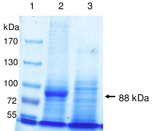
Figure 2 SDS-PAGE analysis Aac expressed by E. coli BL21(DE3). The crude proteins were prepared from the recombinant E. coli BL21 (pET2Iaac) and analysed by 6% SDS-PAGE. The arrow indicates the Aac. Lane 1, pre-stained protein ladder marker; lane 2, IPTG-induced crude proteins; lane 3, IPTG-non-induced crude proteins.
