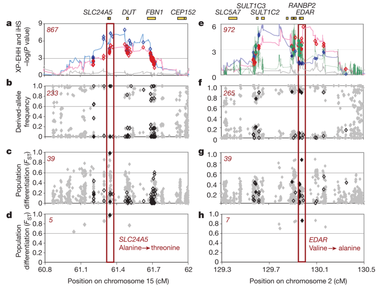
Figure 1. Localizing SLC24A5 and EDAR signals of selection
