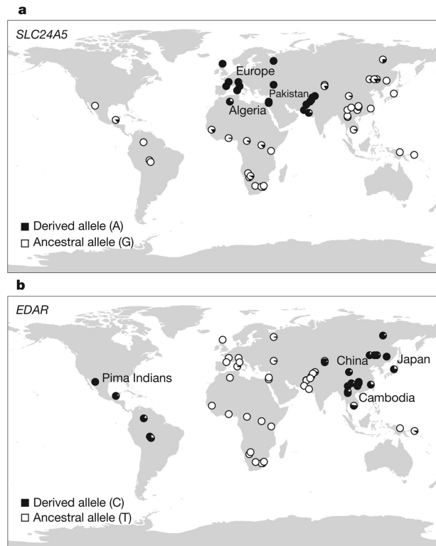
Figure 2. Global distribution of SLC24A5 A111T and EDAR V370A
