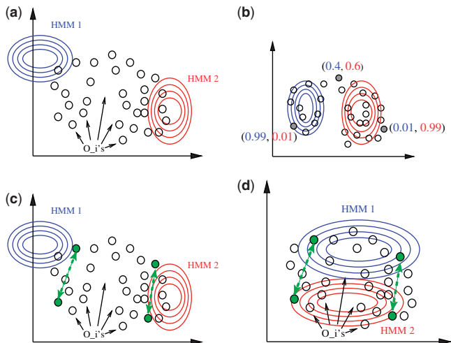
Fig. 2. Schematic illustration of a mixture estimation with and without constraints. (a) The algorithm starts with an initial guess of the mixture components. (b) After termination, the mixture optimally explains the data points. Instead of a hard assignment to the components, each data point has a posterior distribution over the components. (c and d) By including constraints (dashed arrows in green), the EM algorithm strives for an optimum that discriminates the negatively constrained data points.
