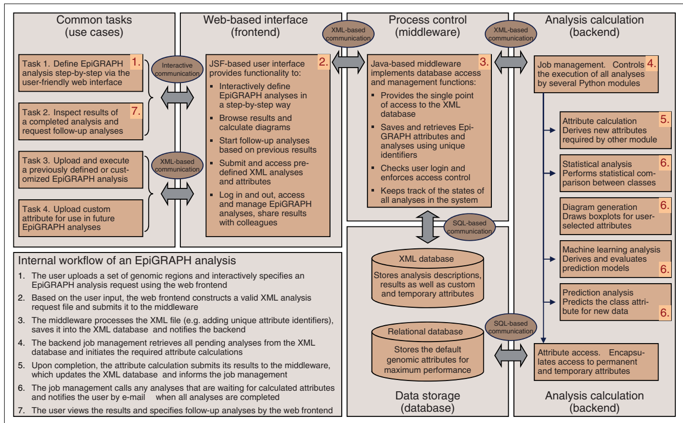
Figure 4 Outline of EpiGRAPH's software architecture. This figure displays a schematic overview of EpiGRAPH's software components, and it describes their interaction in a typical analysis workflow. The red numbers indicate the key component(s) for each step of the workflow description outlined in the bottom left of the figure. JSF, Java Server Faces (which is a Java-based web application framework).
