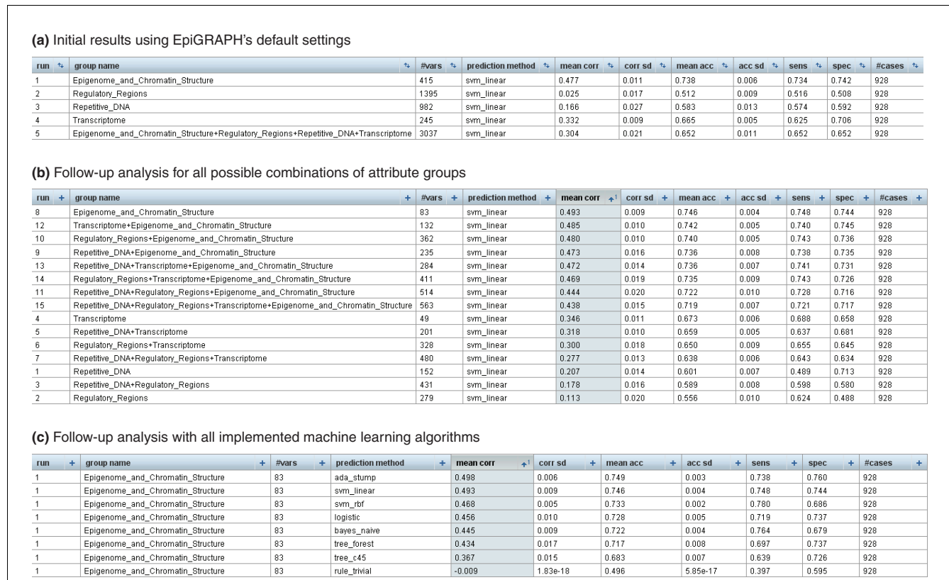
Figure 3 Results screenshots of EpiGRAPH's machine learning module predicting monoallelic gene expression. (a-c) These screenshots display the results of machine learning analyses comparing the promoter regions of monoallelically expressed genes (class = 1) with those of biallelically expressed genes (class = 0), each panel being based on different EpiGRAPH settings. The table values in the tables summarize the average performance of a linear support vector machine or alternative machine learning algorithms (c) that were trained and evaluated in ten repetitions of a tenfold cross-validation. Performance measures include mean correlation ('mean corr' column), prediction accuracy ('mean acc' column), sensitivity ('sens' column) and specificity ('spec' column). Additional columns display standard deviations observed among the repeated cross-validations with random partition assignment ('corr sd' and 'acc sd'), the number of variables in each attribute group ('#vars') and the total number of genomic regions included in the analysis ('#cases').
