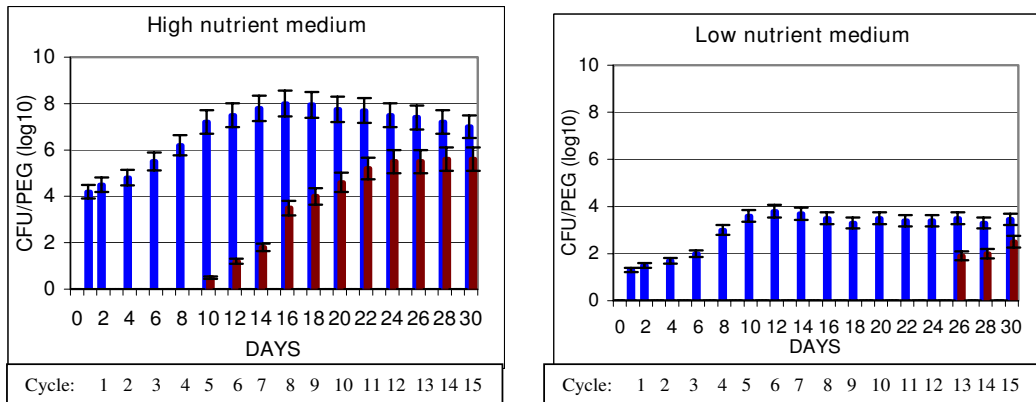
Figure 2 Buildup biofilm (BBF): impact of Glutaraldehyde on microbial survival. P. aeruginosa (a), E. faecalis (b), and C. albicans (c), were used to form BBF in high nutrient medium (enzymatic detergent) or low nutrient medium (tap water). Sample pegs carrying BBF on their surface were removed after varying time periods and the bioburden determined after no treatment (positive control) or after treatment with 2.6% Glutaraldehyde for 20 minutes, where every peg with BBF received multiple cycles of treatment as described in Methods. BBF untreated (blue bar), BBF treated with multiple rounds of drying, Glutaraldehyde, and bioburden exposure (red bar).
