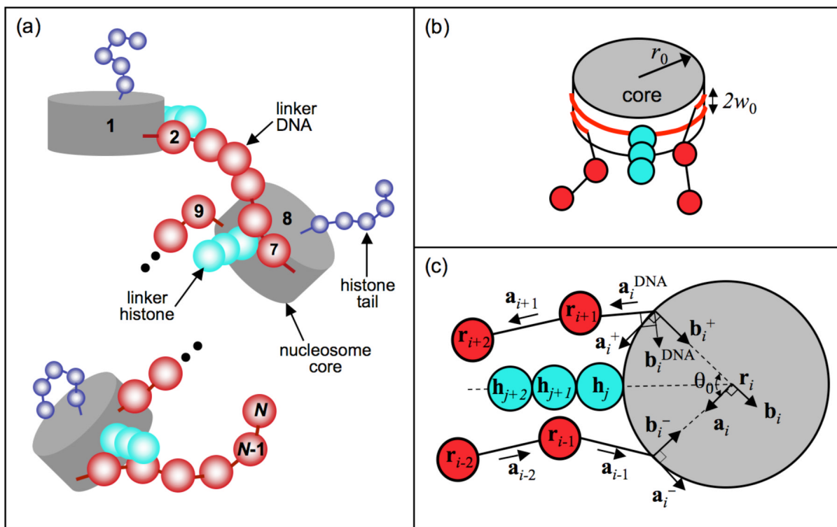
Figure 2. Mesoscale oligonucleosome model showing the: (a) assembly of oligonucleosome motifs into a chain; (b) the entering and exiting linker DNA geometry at the nucleosome core; and (c) the linker-DNA/nucleosome mechanics in terms of individual coordinate systems for the linker DNA beads and the nucleosome core.
