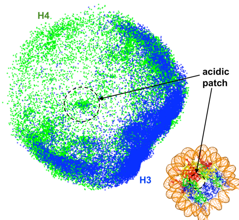
Figure 7. Distribution of the histone tails' (H3, blue and H4, green) attachment sites on the surface of non-parental nucleosomes for MS-LH-Mg conditions. The distributions have been projected onto the plane of the nucleosome. The black circle denotes the acidic patch. The figure in the lower right corner shows the atomistic nucleosome with the same color coding as Fig. 1.
