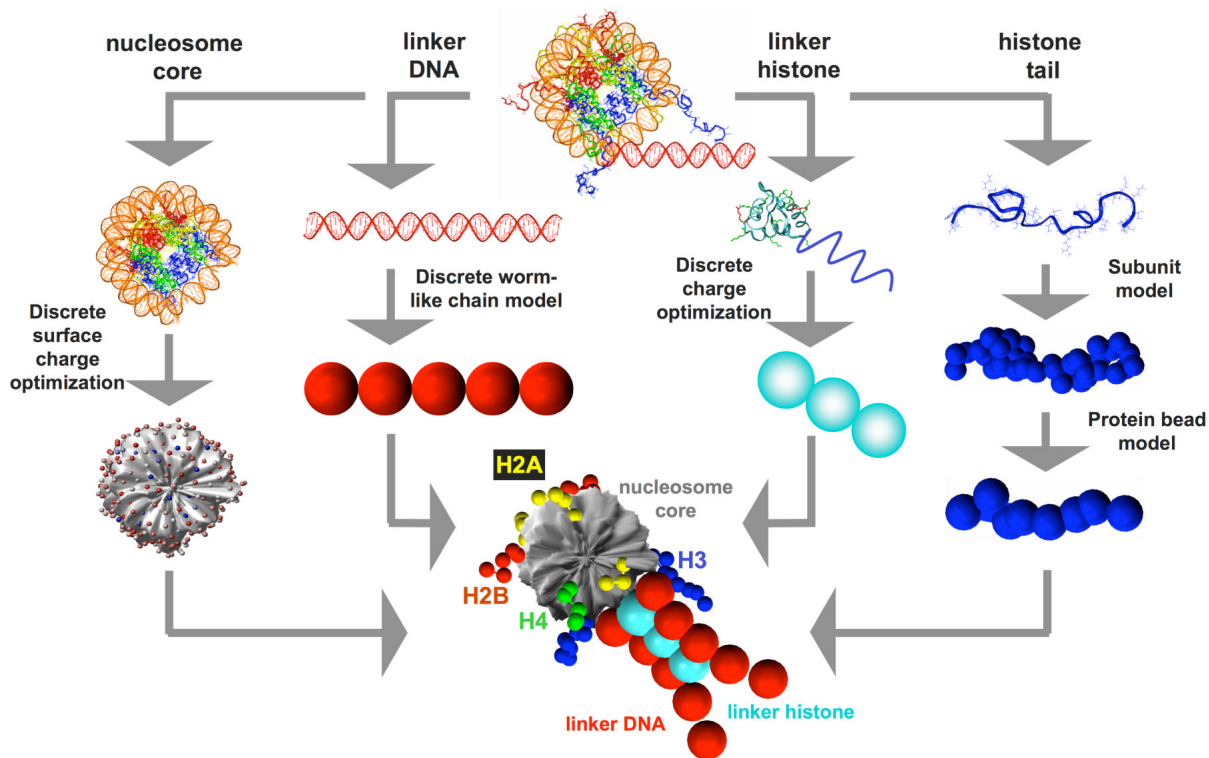
Figure 1. Mesoscale modeling of linker-histone bound oligonucleosomes. The nucleosome core is modeled as an irregular-shaped rigid body with 300 pseudo charges on its surface. The linker DNA is treated using the discrete version of the worm-like chain model. The linker histone is treated as charged beads connected rigidly to the nucleosome and the histone tails are treated using the protein bead model. The bottom figure at center shows the final integrated mesoscale model.
