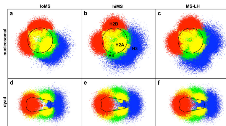
Figure 5. Positional distribution of histone tails under different conditions: low monovalent salt (a,d); high monovalent salt (b,e); and high monovalent salt with bound linker histones (c,f). The upper panel (a-c) represents the histone tail positions projected onto the nucleosomal plane of the parent nucleosomes, and the lower panel (e-f) represents the positions projected onto the dyad plane of the parent nucleosomes. The tails are colored as: H2A, yellow; H2B, red; H3, blue; and H4, green. The nucleosome boundaries are indicated by the solid black lines.
