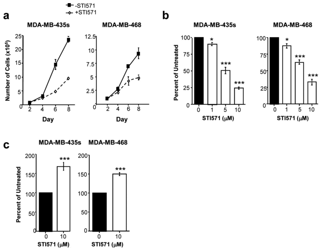
Fig. 1. STI571 inhibits cell growth, proliferation, and induces apoptosis of cells containing highly active Abl kinases
