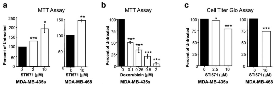
Fig. 2. STI571 interferes with the ability of the MTT assay to measure cell viability MDA-MB-435s melanoma cells and MDA-MB-468 breast cancer cells were plated in 96-well dishes in triplicate, the media was replaced the next day with media containing STI571 (a,c) or doxorubicin (b), and 72 hours later the cells were used either in MTT (a,b) or Cell Titer Glo (c) viability assays. Experiments shown are mean \pm s.e.m. for three independent experiments. * p < 0.05 , ** p < 0.005 , *** p < 0.001 using Student t-tests. Some error bars are too small to be visualized.
