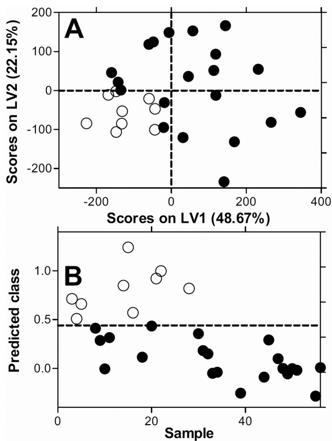
Figure 3. Partial least squares discriminant analysis (PLS-DA) of vitreous fluid NMR spectra from lens-induced uveitis and chronic uveitis patients. A: PLS-DA model was constructed to predict diagnostic groups. A: Latent variable plot of the PLS-DA model, showing improved discrimination between LIU and chronic uveitis compared with the PCA analysis (Figure 2). B: Prediction of the group membership from the PLS-DA. The model was cross validated, and was able to predict the classes, LIU and chronic uveitis, with sensitivity of 78% and specificity of 85%.
