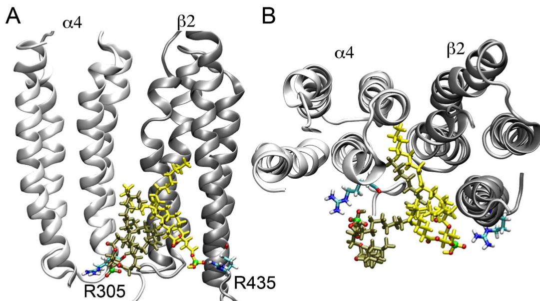
Figure 2. (A) Side view of two POPA lipids forming salt bridges with two adjacent Arg residues ( \alpha 4 -R305 and \beta 2 -R435); and (B) Top-view of these two POPA lipids penetrating into an inter-subunit protein cavity between the \alpha 4 (white) and \beta 2 (silver) subunits. Two POPA lipids (colored in yellow and tan) are shown in licorice format with oxygen and phosphor atoms highlighted in red and green, respectively. Arg residues are plotted in licorice format. Nitrogen, oxygen, hydrogen, and carbon atoms are shown in blue, red, white, and cyan, respectively.
