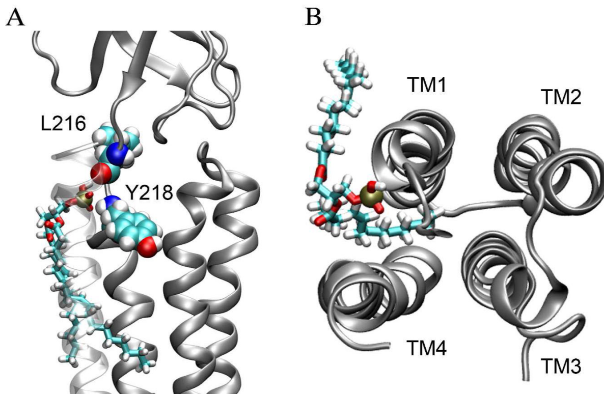
Figure 4. (A) Side view of a POPA lipid bound to a putative binding pocket near the pre-TM1 segment in the \alpha 4 subunit; and (B) top view of the POPA lipid penetrating into an intra-subunit protein pocket. The POPA lipid is shown in licorice format and the protein subunit is shown in silver. Nitrogen, oxygen, hydrogen, phosphor, and carbon atoms are shown in blue, red, white, tan, and cyan, respectively.
