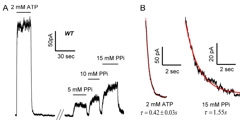
Figure 1. The effect of Mg PPi on WT-CFTR. (A) A recording of WT-CFTR channels in an excised inside-out membrane patch. The channels were activated by 2 mM ATP plus 25 U/ml PKA (not depicted). After phosphorylation-dependent activation, application and removal of ATP result in rapid current rise and decay, respectively. 3 min after washout of ATP, channels were opened by different concentrations of PPi plus Mg 2+ . 15 mM PPi supplemented with 15 mM MgPPi still seems unable to saturate the macroscopic current. (B) Macroscopic current decay after ATP withdrawal (left) and the ensemble current relaxation after washout of 15 mM MgPPi (right). Channels opened by MgPPi appear to close more slowly than those opened by ATP.
