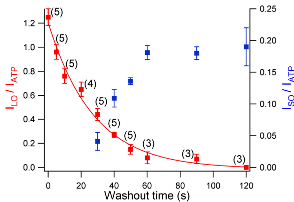
Figure 4. Time-dependent reopening of WT-CFTR by 10 mM MgPPi. Mg PPI was applied at different time points after ATP washout. The current amplitude of the slow component (red squares, left y axis) and the fast component (blue squares, right y axis) derived from double-exponential fitting were normalized to ATP current at t = 0 . For t = 0 \sim 20 s, the fast component was too small to be resolved. Fitting the data points (red curve) by a single-exponential function estimates the lifetime of the C_2 state to be 27.4 s.
