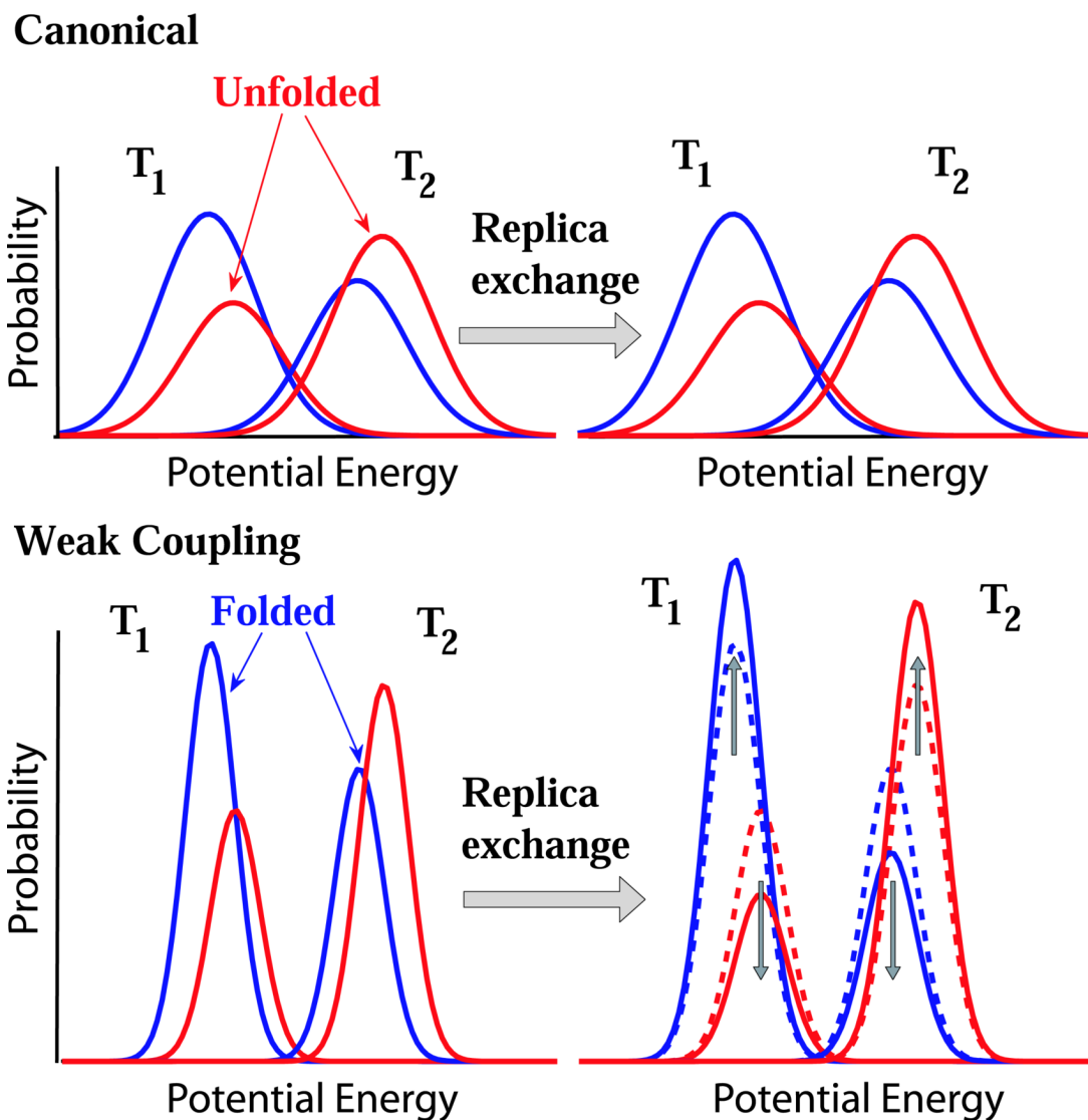
Figure 4. Schematic of the effect of REMD with W-C thermostats on folding probabilities. Potential energy probability distributions of folded (blue) and unfolded (red) states are shown at two temperatures before and after replica exchange. For classical canonical distributions (upper panel), REMD does not affect the distributions. However, for the narrowed distributions in W-C REMD (lower panel), replica exchange alters the relative populations of folded and unfolded states. Folded states become overpopulated at low temperatures and underpopulated at high temperatures, as indicated by the vertical arrows.
