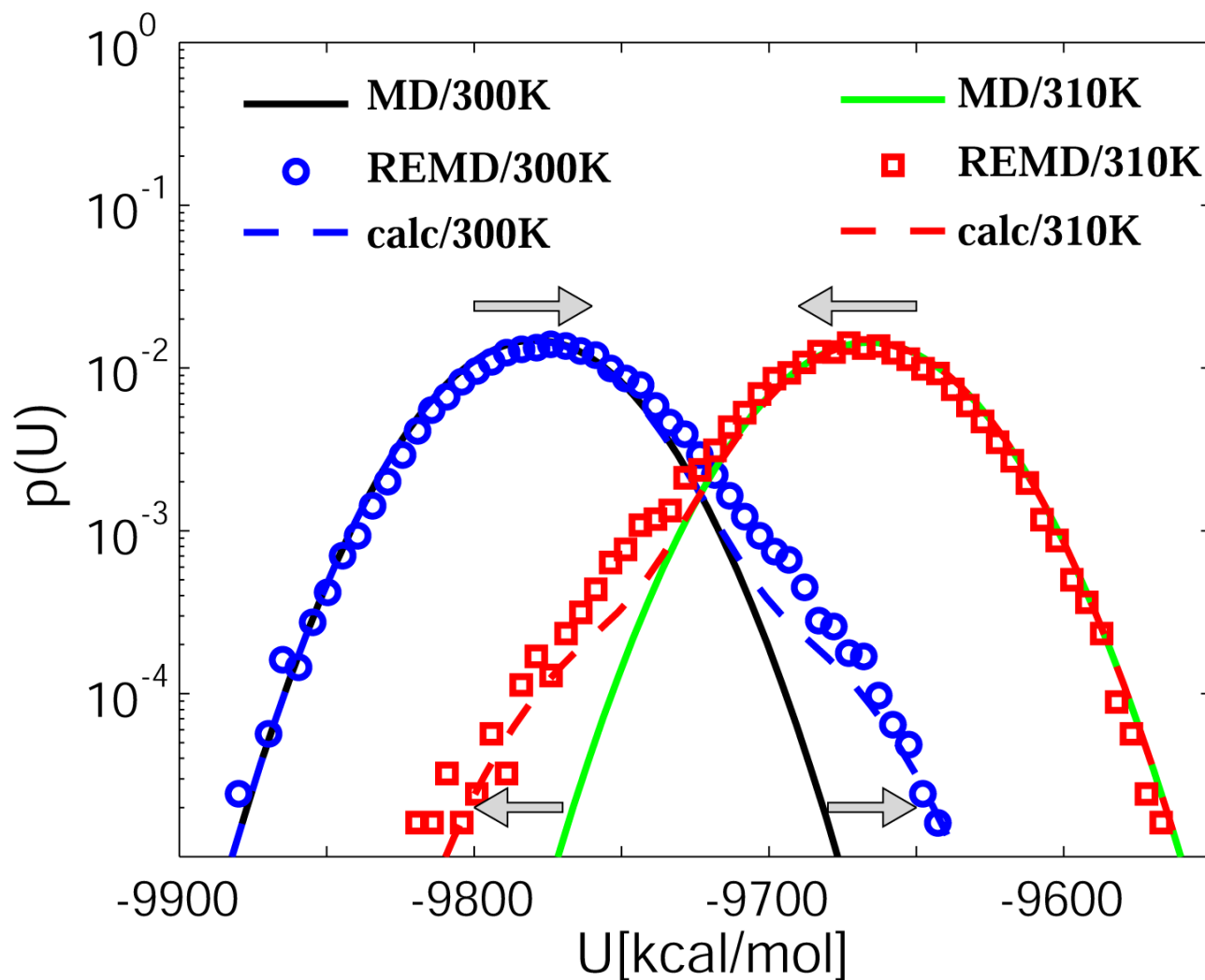
Figure 2. Comparison of bulk TIP3P water potential energy distributions from MD and REMD simulations (semi-logarithmic scale). The blue circles and red squares show the REMD results for the replicas at 300 and 310 K, respectively. The blue and red dashed lines are calculated from iterated numerical solutions of eq 2 at 300 and 310 K, respectively. For reference, Gaussian approximations to the MD results using a W-C thermostat 4 with a coupling time of 5 ps are shown as black (300 K) and green lines (310 K). The arrows indicate the change in the energy distributions of REMD simulations compared to MD, in particular the buildup of artificial tails and the small shifts in the means.
