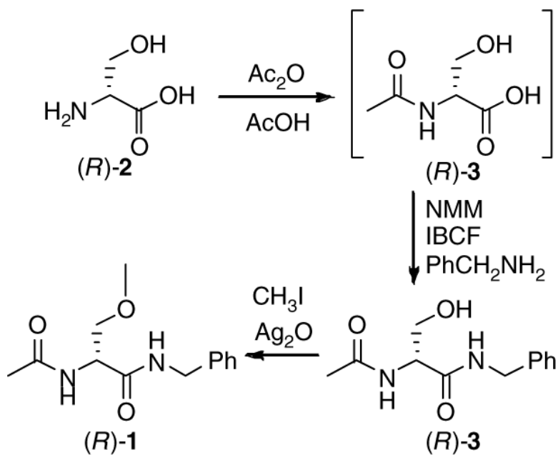
Scheme 1. Three-step synthesis of (R)-lacosamide (1).
