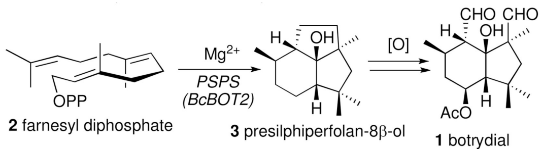
Scheme 1. Biosynthesis of Botrydial ( 1 ).
