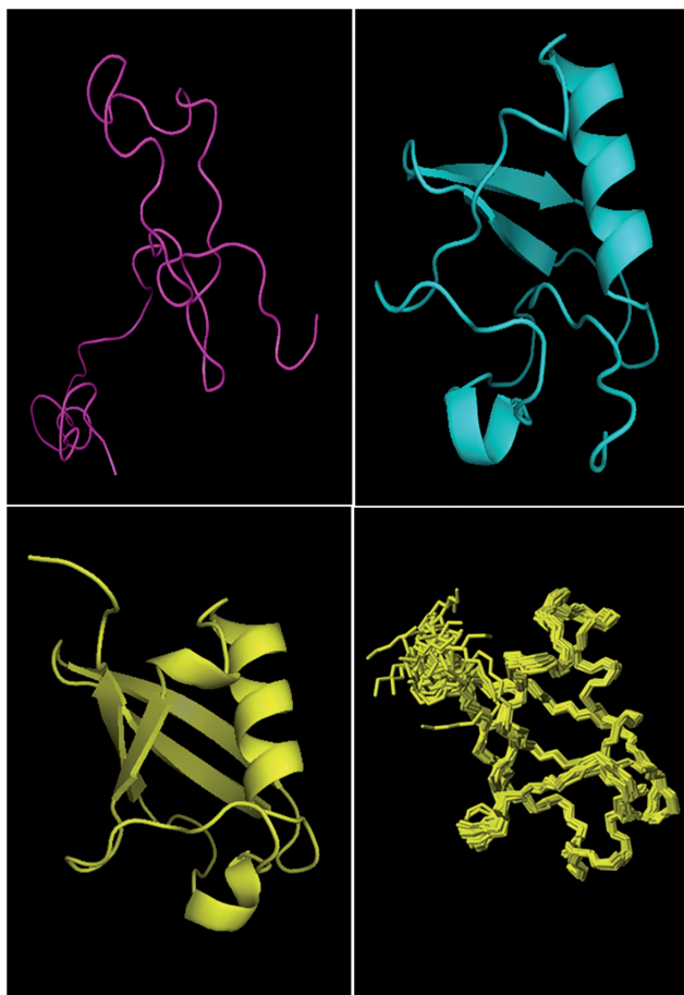
Figure 2. Illustration of how GeNMR is able to generate the structure of ubiquitin using only experimental NOE constraints [scenario (d) in the article]. The initial structure (purple) is a largely random coil polypeptide ( \sim 18 Å RMSD), an intermediate structure (cyan) contains most of the secondary structure elements ( \sim 3.9 Å RMSD), while the lowest energy structure (yellow), refined via simulated annealing, is within 1.2 Å of the known X-ray structure. The last panel shows the final ensemble (or bundle) of structures generated by GeNMR.
