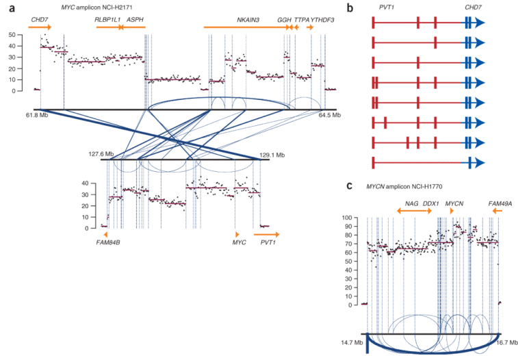
Figure 5. Amplicons in NCI-H2171 and NCI-H1770. (a) The MYC amplicon of NCI-H2171 involves two regions of chromosome 8q, both of which show extensive variation in copy number. Breakpoints between and within the two regions are shown in blue lines, with the thickness of the line proportional to the number of paired-end reads spanning the same breakpoint. The locations of the breakpoints frequently correspond to changes in copy number. (b) A PVT1-CHD7 fusion gene is created by the most commonly seen breakpoint in the MYC amplicon. Extensive splicing of the PVT1 moiety was seen on RT-PCR, but the three most common transcripts accounted for 23 of 30 of colonies sequenced. (c) The NMYC amplicon of NCI-H1770 showed up to 85-fold amplification of a 2-Mb region. The most common breakpoint observed demarcated the 5' and 3' borders of the amplicon and suggested tandem insertion of the 2-Mb region, but several other rearrangements were seen within the amplicon, both inverted (arcs above the line) and noninverted (arcs below the line).
