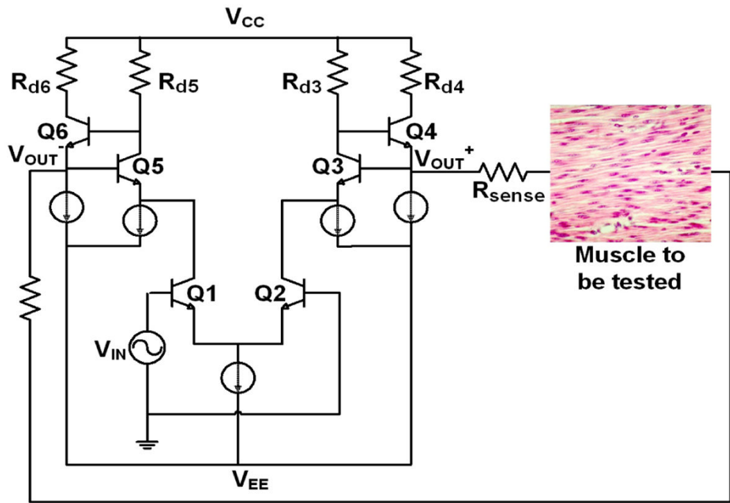
Fig. 3. Differential Voltage Driver.
