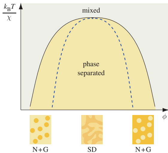
Figure 3. A schematic phase diagram showing the relationship between the temperature ( k_B T/\chi ), composition ( \phi ) and the stability of a mixture. k_B is Boltzmann's constant, T is the absolute temperature and \chi is the strength of interactions between dissimilar molecules. In feathers, \phi would represent the volume fraction of \beta -keratin. At high-temperature conditions, a molecular mixture will be stable at any composition, but below the phase-separation boundary (solid line) the solution will phase separate. Mixtures below the spinodal line (dashed line) are unstable, and will phase separate by SD, which produces bicontinuous channels of each material (middle inset). Mixtures between the spinodal line and the phase boundary are metastable, and will only phase separate through nucleation and growth (N+G), which produces spherical shapes (left and right insets).
